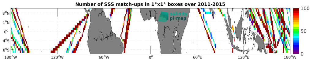
Figure 4: Number of SSS match-ups between TSG (LEGOS-DM) SSS and the Aquarius SSS L3 OR v5 - 7-Day running (NASA-GSFC) SSS product for the Equatorial Ocean 10N-10S Pi-MEP region over 1^\circ \times 1^\circ boxes and for the full satellite product period.
