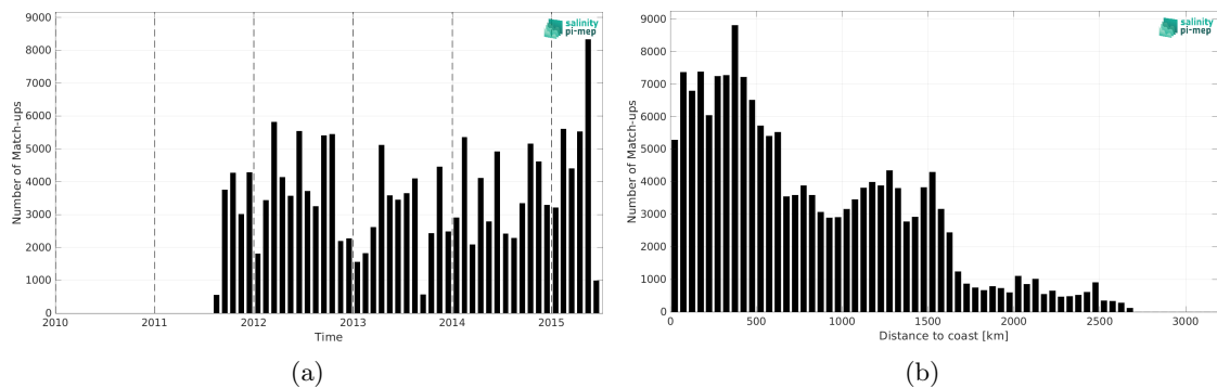
Figure 1: Number of match-ups between TSG (LEGOS-DM) and Aquarius SSS L3 OR v5 - 7-Day running (NASA-GSFC) SSS as a function of time (a) and as function of the distance to coast (b) over the Equatorial Ocean 10N-10S Pi-MEP region and for the full satellite product period.
