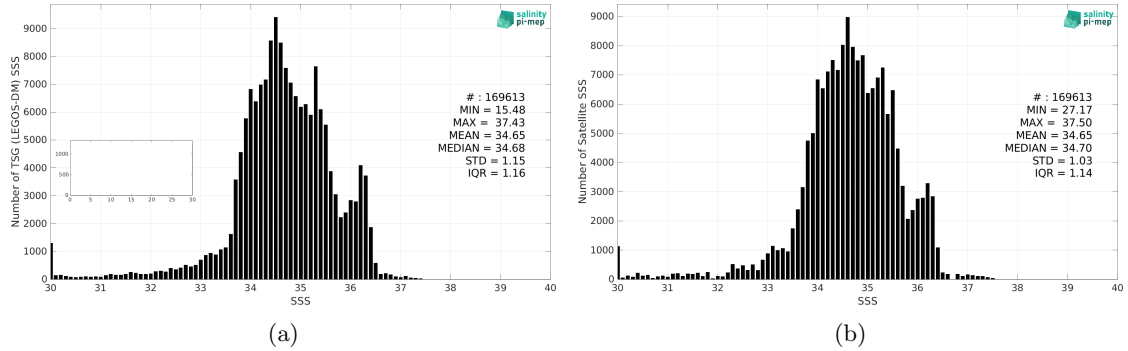
Figure 2: Histograms of SSS from TSG (LEGOS-DM) (a) and Aquarius SSS L3 OR v5 - 7-Day running (NASA-GSFC) (b) considering all match-up pairs per bins of 0.1 over the Equatorial Ocean 10N-10S Pi-MEP region and for the full satellite product period.
