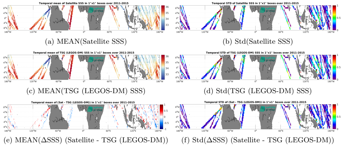
Figure 6: Temporal mean (left) and Std (right) of SSS from Aquarius SSS L3 OR v5 - 7-Day running (NASA-GSFC) (top), TSG (LEGOS-DM) (middle), and of \Delta SSS (Satellite - TSG (LEGOS-DM)). Only match-up pairs are used to generate these maps.
