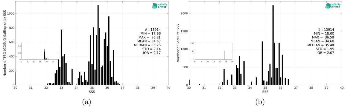
Figure 3: Histograms of SSS from TSG (GOSUD-Sailing-ship) (a) and Aquarius SSS L3 OR v5 - 7-Day running (NASA-GSFC) (b) considering all match-up pairs per bins of 0.1 over the Equatorial Ocean 10N-10S Pi-MEP region and for the full satellite product period.
