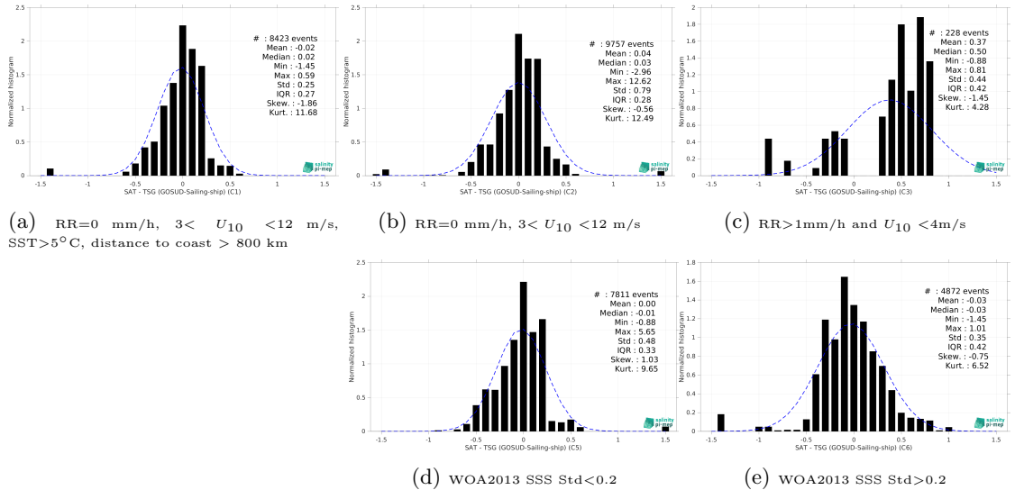
Figure 15: Normalized histogram of \Delta SSS (Aquarius SSS L3 OR v5 - 7-Day running (NASA-GSFC) - TSG (GOSUD-Sailing-ship)) for 5 different subdatasets corresponding to: RR=0 mm/h, 3 < U_{10} < 12 m/s, SST>5°C, distance to coast > 800 km (a), RR=0 mm/h, 3 < U_{10} < 12 m/s (b), RR>1mm/h and U_{10} < 4 m/s (c), WOA2013 SSS Std<0.2 (d), WOA2013 SSS Std>0.2 (e).
