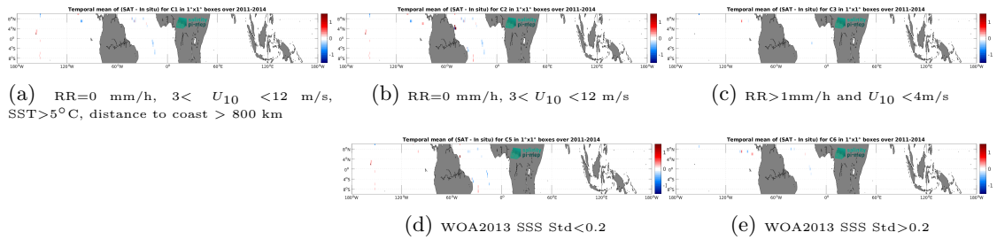
Figure 14: Temporal mean gridded over spatial boxes of size 1^\circ \times 1^\circ of \Delta SSS (Aquarius SSS L3 OR v5 - 7-Day running (NASA-GSFC) - TSG (GOSUD-Sailing-ship)) for 5 different subdatasets corresponding to:RR=0 mm/h, 3 < U_{10} < 12 m/s, SST>5°C, distance to coast > 800 km (a), RR=0 mm/h, 3 < U_{10} < 12 m/s (b), RR>1mm/h and U_{10} < 4 m/s (c), WOA2013 SSS Std<0.2 (d), WOA2013 SSS Std>0.2 (e).
