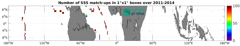
Figure 5: Number of SSS match-ups between TSG (GOSUD-Sailing-ship) SSS and the Aquarius SSS L3 OR v5 - 7-Day running (NASA-GSFC) SSS product for the Equatorial Ocean 10N-10S Pi-MEP region over 1^\circ \times 1^\circ boxes and for the full satellite product period.
