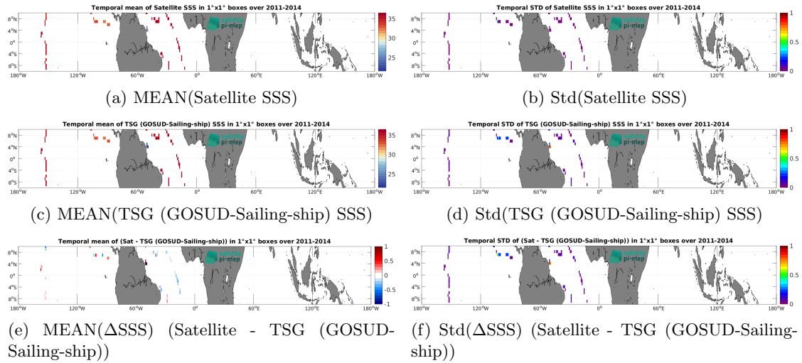
Figure 7: Temporal mean (left) and Std (right) of SSS from Aquarius SSS L3 OR v5 - 7-Day running (NASA-GSFC) (top), TSG (GOSUD-Sailing-ship) (middle), and of \Delta SSS (Satellite - TSG (GOSUD-Sailing-ship)). Only match-up pairs are used to generate these maps.
