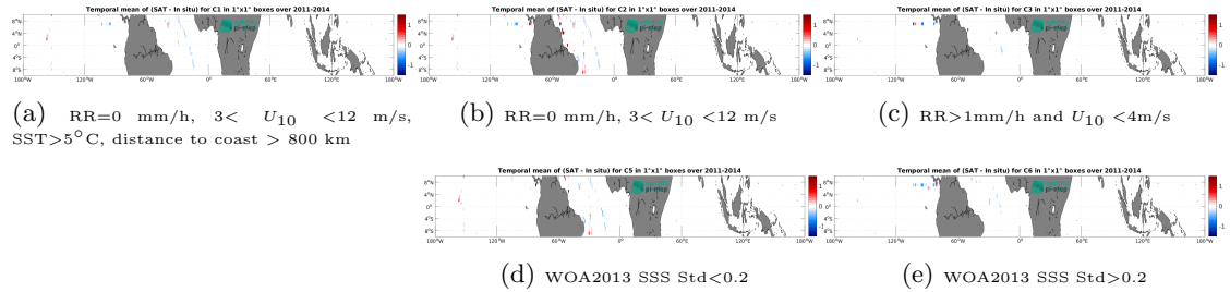
Figure 12: Temporal mean gridded over spatial boxes of size 1^{\circ}\times 1^{\circ} of \Delta SSS (Aquarius SSS L3 OR v5 - 7-Day running (NASA-GSFC) - TSG (GOSUD-Sailing-ship)) for 5 different subdatasets corresponding to:RR=0 mm/h, 3 < U_{10} < 12 m/s, SST >5^{\circ}\text{C} , distance to coast > 800 km (a), RR=0 mm/h, 3 < U_{10} < 12 m/s (b), RR >1 mm/h and U_{10} < 4 m/s (c), WOA2013 SSS Std <0.2 (d), WOA2013 SSS Std >0.2 (e).
