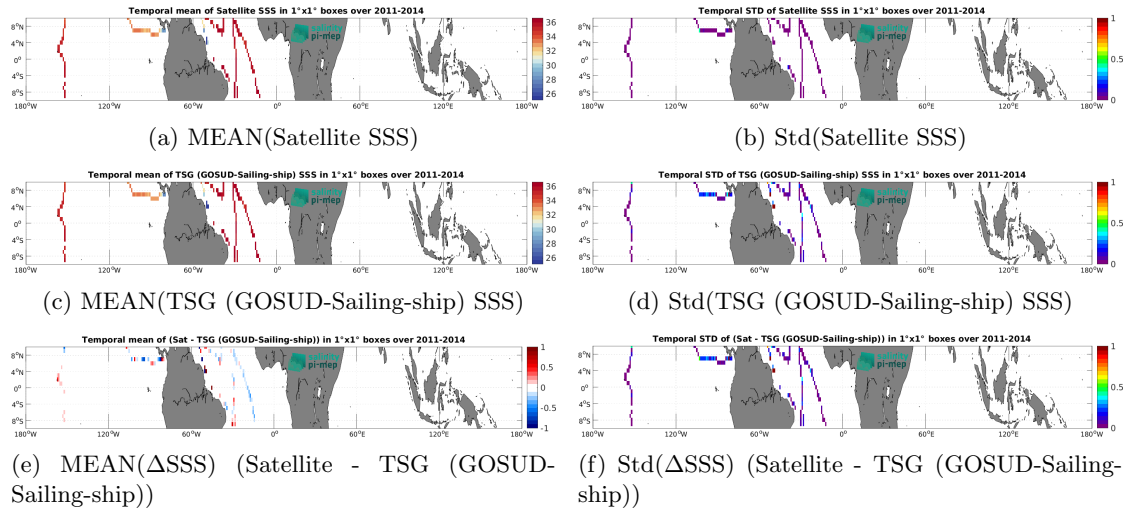
Figure 6: Temporal mean (left) and Std (right) of SSS from Aquarius SSS L3 OR v5 - 7-Day running (NASA-GSFC) (top), TSG (GOSUD-Sailing-ship) (middle), and of \Delta SSS (Satellite - TSG (GOSUD-Sailing-ship)). Only match-up pairs are used to generate these maps.
