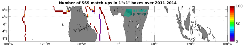
Figure 4: Number of SSS match-ups between TSG (GOSUD-Sailing-ship) SSS and the Aquarius SSS L3 OR v5 - 7-Day running (NASA-GSFC) SSS product for the Equatorial Ocean 10N-10S Pi-MEP region over 1^\circ \times 1^\circ boxes and for the full satellite product period.
