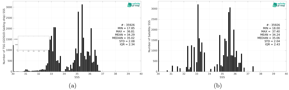
Figure 2: Histograms of SSS from TSG (GOSUD-Sailing-ship) (a) and Aquarius SSS L3 OR v5 - 7-Day running (NASA-GSFC) (b) considering all match-up pairs per bins of 0.1 over the Equatorial Ocean 10N-10S Pi-MEP region and for the full satellite product period.
