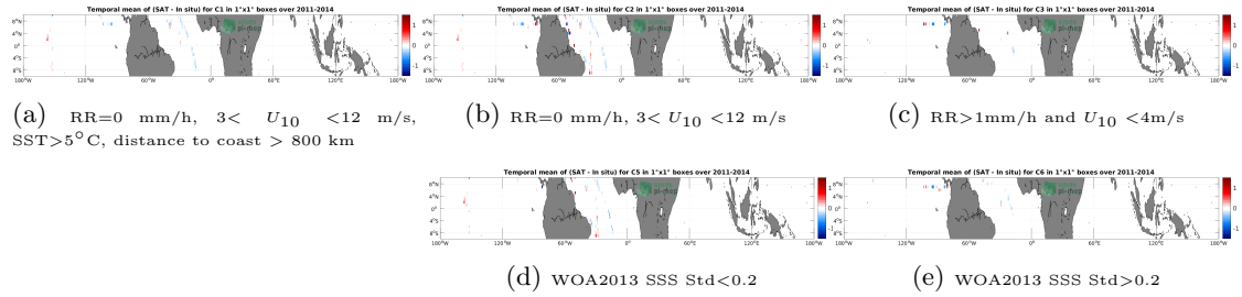
Figure 12: Temporal mean gridded over spatial boxes of size 1^\circ \times 1^\circ of \Delta SSS (Aquarius SSS L3 OR v5 - 7-Day running (NASA-GSFC) - TSG (GOSUD-Sailing-ship)) for 5 different subdatasets corresponding to:RR=0 mm/h, 3 < U_{10} < 12 m/s, SST >5^\circ\text{C} , distance to coast > 800 km (a), RR=0 mm/h, 3 < U_{10} < 12 m/s (b), RR >1 mm/h and U_{10} < 4 m/s (c), WOA2013 SSS Std <0.2 (d), WOA2013 SSS Std >0.2 (e).
