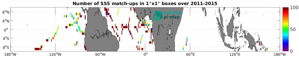
Figure 5: Number of SSS match-ups between TSG (GOSUD-Research-vessel) SSS and the Aquarius SSS L3 OR v5 - 7-Day running (NASA-GSFC) SSS product for the Equatorial Ocean 10N-10S Pi-MEP region over 1^\circ \times 1^\circ boxes and for the full satellite product period.
