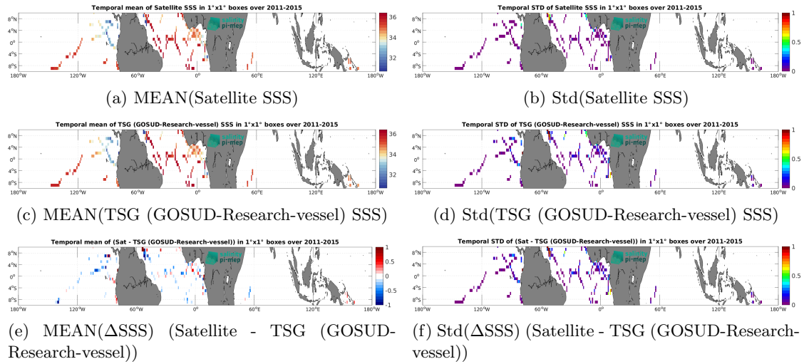
Figure 7: Temporal mean (left) and Std (right) of SSS from Aquarius SSS L3 OR v5 - 7-Day running (NASA-GSFC) (top), TSG (GOSUD-Research-vessel) (middle), and of \Delta SSS (Satellite - TSG (GOSUD-Research-vessel)). Only match-up pairs are used to generate these maps.
