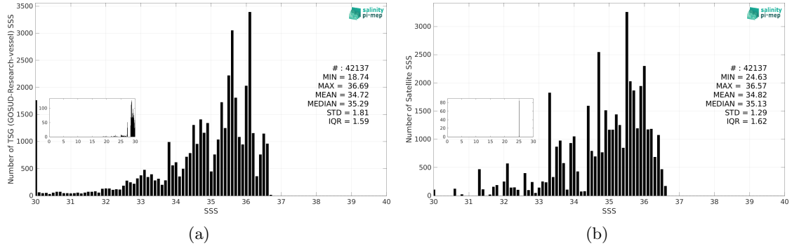
Figure 3: Histograms of SSS from TSG (GOSUD-Research-vessel) (a) and Aquarius SSS L3 OR v5 - 7-Day running (NASA-GSFC) (b) considering all match-up pairs per bins of 0.1 over the Equatorial Ocean 10N-10S Pi-MEP region and for the full satellite product period.
