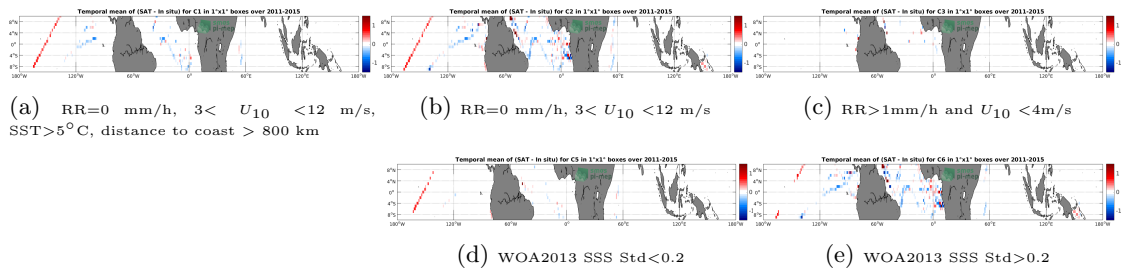
Figure 12: Temporal mean gridded over spatial boxes of size 1^\circ \times 1^\circ of \Delta SSS (Aquarius-L3-OR-V5-7DAY-RUNNING-1DEG - TSG-GOSUD-Research-vessel) for 5 different subdatasets corresponding to:RR=0 mm/h, 3 < U_{10} < 12 m/s, SST > 5^\circ C , distance to coast > 800 km (a), RR=0 mm/h, 3 < U_{10} < 12 m/s (b), RR >1 mm/h and U_{10} < 4 m/s (c), WOA2013 SSS Std <0.2 (d), WOA2013 SSS Std >0.2 (e).
