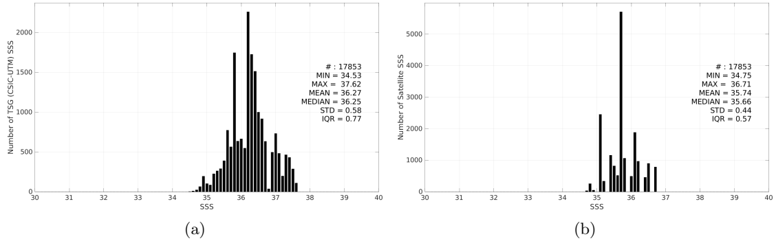
Figure 3: Histograms of SSS from TSG (CSIC-UTM) (a) and Aquarius SSS L3 OR v5 - 7-Day running (NASA-GSFC) (b) considering all match-up pairs per bins of 0.1 over the Equatorial Ocean 10N-10S Pi-MEP region and for the full satellite product period.
