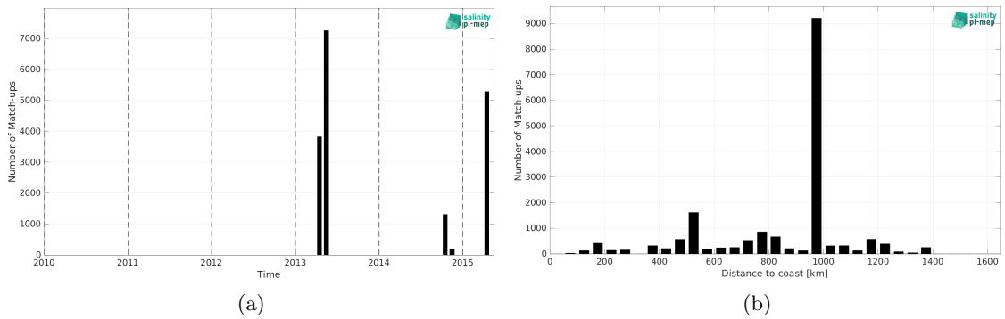
Figure 2: Number of match-ups between TSG (CSIC-UTM) and Aquarius SSS L3 OR v5 - 7-Day running (NASA-GSFC) SSS as a function of time (a) and as function of the distance to coast (b) over the Equatorial Ocean 10N-10S Pi-MEP region and for the full satellite product period.
