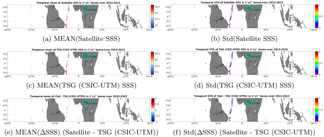
Figure 7: Temporal mean (left) and Std (right) of SSS from Aquarius SSS L3 OR v5 - 7-Day running (NASA-GSFC) (top), TSG (CSIC-UTM) (middle), and of \Delta SSS (Satellite - TSG (CSIC-UTM)). Only match-up pairs are used to generate these maps.
