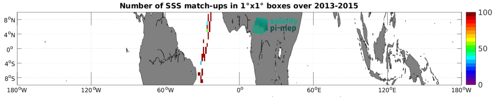
Figure 5: Number of SSS match-ups between TSG (CSIC-UTM) SSS and the Aquarius SSS L3 OR v5 - 7-Day running (NASA-GSFC) SSS product for the Equatorial Ocean 10N-10S Pi-MEP region over 1^\circ \times 1^\circ boxes and for the full satellite product period.
