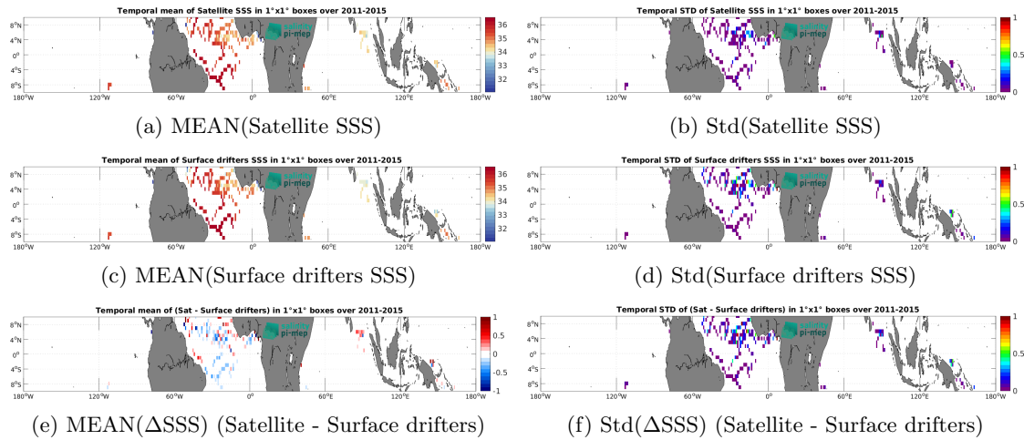
Figure 6: Temporal mean (left) and Std (right) of SSS from Aquarius SSS L3 OR v5 - 7-Day running (NASA-GSFC) (top), Surface drifters (middle), and of \Delta SSS (Satellite - Surface drifters). Only match-up pairs are used to generate these maps.
