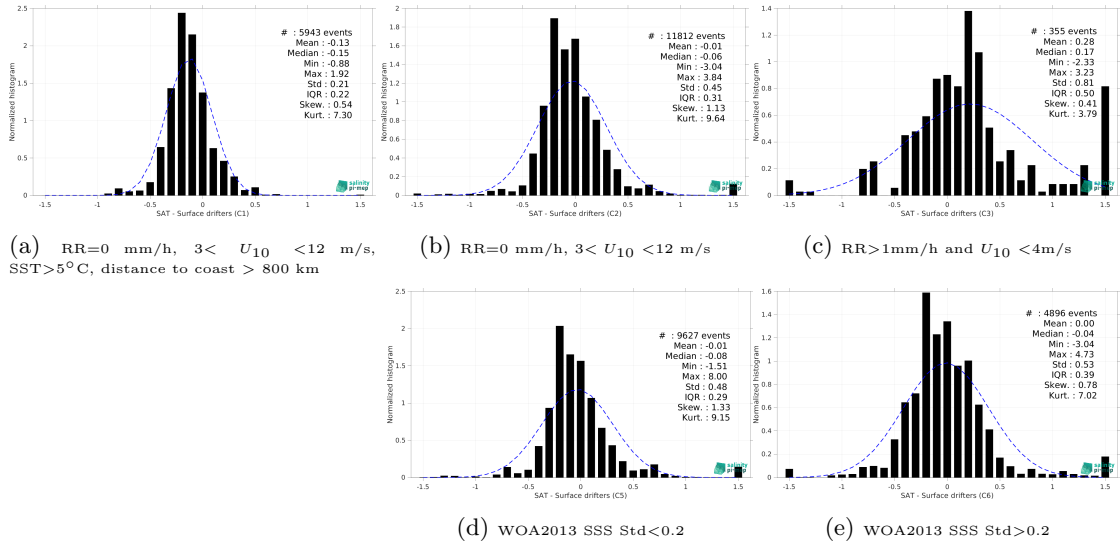
Figure 14: Normalized histogram of \Delta SSS (Aquarius SSS L3 OR v5 - 7-Day running (NASA-GSFC) - Surface drifters) for 5 different subdatasets corresponding to: RR=0 mm/h, 3 < U_{10} < 12 m/s, SST >5^\circ\text{C} , distance to coast > 800 km (a), RR=0 mm/h, 3 < U_{10} < 12 m/s (b), RR >1 mm/h and U_{10} < 4 m/s (c), WOA2013 SSS Std <0.2 (d), WOA2013 SSS Std >0.2 (e).
