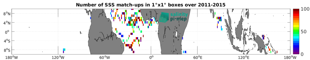
Figure 4: Number of SSS match-ups between Surface drifters SSS and the Aquarius SSS L3 OR v5 - 7-Day running (NASA-GSFC) SSS product for the Equatorial Ocean 10N-10S Pi-MEP region over 1^\circ \times 1^\circ boxes and for the full satellite product period.
