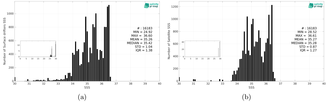
Figure 3: Histograms of SSS from Surface drifters (a) and Aquarius SSS L3 OR v5 - 7-Day running (NASA-GSFC) (b) considering all match-up pairs per bins of 0.1 over the Equatorial Ocean 10N-10S Pi-MEP region and for the full satellite product period.
