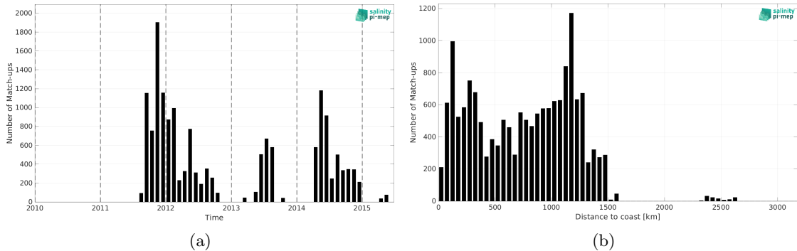
Figure 2: Number of match-ups between Surface drifters and Aquarius SSS L3 OR v5 - 7-Day running (NASA-GSFC) SSS as a function of time (a) and as function of the distance to coast (b) over the Equatorial Ocean 10N-10S Pi-MEP region and for the full satellite product period.
