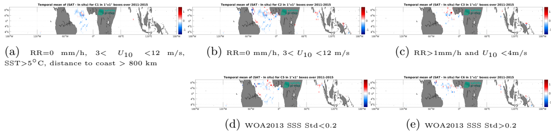
Figure 11: Temporal mean gridded over spatial boxes of size 1^\circ \times 1^\circ of \Delta SSS (Aquarius SSS L3 OR v5 - 7-Day running (NASA-GSFC) - Surface drifters) for 5 different subdatasets corresponding to: RR=0 mm/h, 3 < U_{10} < 12 m/s, SST >5^\circ\text{C} , distance to coast > 800 km (a), RR=0 mm/h, 3 < U_{10} < 12 m/s (b), RR >1 mm/h and U_{10} < 4 m/s (c), WOA2013 SSS Std <0.2 (d), WOA2013 SSS Std >0.2 (e).
