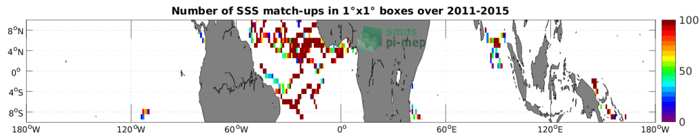
Figure 3: Number of SSS match-ups between Surface drifters SSS and the Aquarius SSS L3 OR v5 - 7-Day running (NASA-GSFC) SSS product for the Equatorial Ocean 10N-10S Pi-MEP region over 1^\circ \times 1^\circ boxes and for the full satellite product period.
