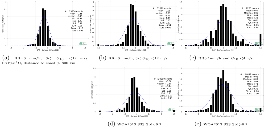
Figure 12: Normalized histogram of \Delta SSS (Aquarius SSS L3 OR v5 - 7-Day running (NASA-GSFC) - Surface drifters) for 5 different subdatasets corresponding to: RR=0 mm/h, 3 < U_{10} < 12 m/s, SST >5^\circ\text{C} , distance to coast > 800 km (a), RR=0 mm/h, 3 < U_{10} < 12 m/s (b), RR >1 mm/h and U_{10} < 4 m/s (c), WOA2013 SSS Std <0.2 (d), WOA2013 SSS Std >0.2 (e).
