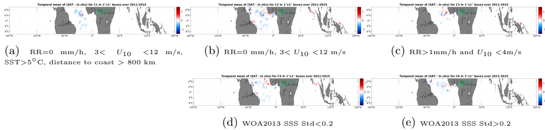
Figure 11: Temporal mean gridded over spatial boxes of size 1^\circ \times 1^\circ of \Delta SSS (Aquarius SSS L3 OR v5 - 7-Day running (NASA-GSFC) - Surface drifters) for 5 different subdatasets corresponding to: RR=0 mm/h, 3 < U_{10} < 12 m/s, SST >5^\circ\text{C} , distance to coast > 800 km (a), RR=0 mm/h, 3 < U_{10} < 12 m/s (b), RR >1 mm/h and U_{10} < 4 m/s (c), WOA2013 SSS Std <0.2 (d), WOA2013 SSS Std >0.2 (e).
