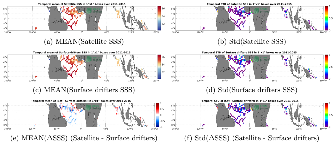
Figure 5: Temporal mean (left) and Std (right) of SSS from Aquarius SSS L3 OR v5 - 7-Day running (NASA-GSFC) (top), Surface drifters (middle), and of \Delta SSS (Satellite - Surface drifters). Only match-up pairs are used to generate these maps.
