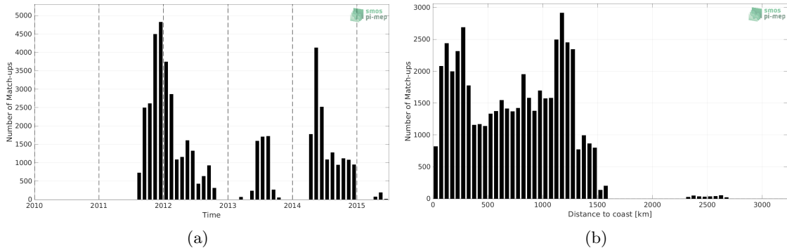
Figure 1: Number of match-ups between Surface drifters and Aquarius SSS L3 OR v5 - 7-Day running (NASA-GSFC) SSS as a function of time (a) and as function of the distance to coast (b) over the Equatorial Ocean 10N-10S Pi-MEP region and for the full satellite product period.
