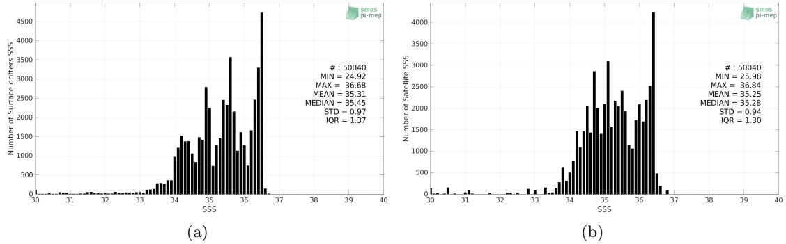
Figure 2: Histograms of SSS from Surface drifters (a) and Aquarius SSS L3 OR v5 - 7-Day running (NASA-GSFC) (b) considering all match-up pairs per bins of 0.1 over the Equatorial Ocean 10N-10S Pi-MEP region and for the full satellite product period.
