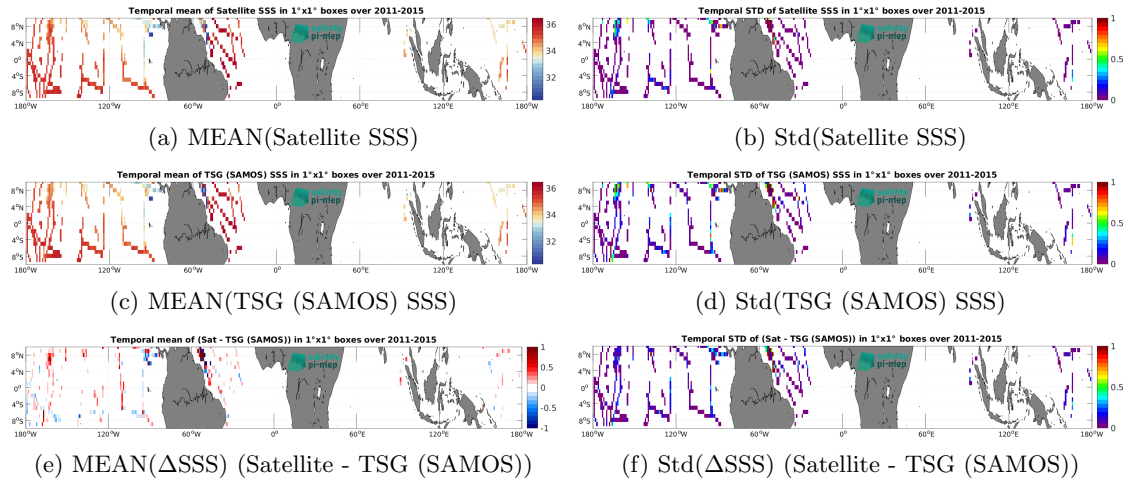
Figure 7: Temporal mean (left) and Std (right) of SSS from Aquarius SSS L3 OR v5 - 7-Day running - Rain mask (NASA-GSFC) (top), TSG (SAMOS) (middle), and of \Delta SSS (Satellite - TSG (SAMOS)). Only match-up pairs are used to generate these maps.
