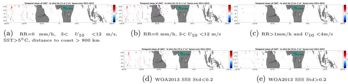
Figure 14: Temporal mean gridded over spatial boxes of size 1^\circ \times 1^\circ of \Delta SSS (Aquarius SSS L3 OR v5 - 7-Day running - Rain mask (NASA-GSFC) - TSG (SAMOS)) for 5 different subdatasets corresponding to: RR=0 mm/h, 3 < U_{10} < 12 m/s, SST>5°C, distance to coast > 800 km (a), RR=0 mm/h, 3 < U_{10} < 12 m/s (b), RR>1mm/h and U_{10} < 4 m/s (c), WOA2013 SSS Std<0.2 (d), WOA2013 SSS Std>0.2 (e).
