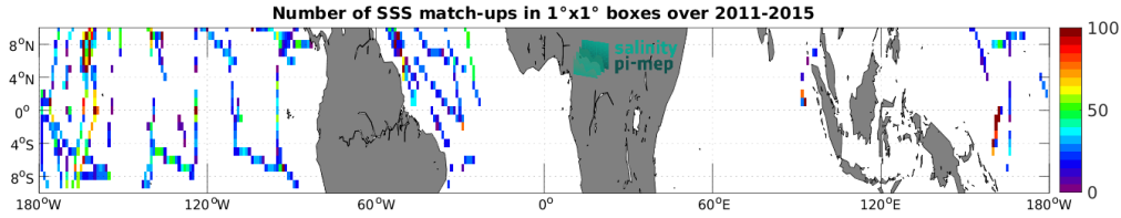
Figure 5: Number of SSS match-ups between TSG (SAMOS) SSS and the Aquarius SSS L3 OR v5 - 7-Day running - Rain mask (NASA-GSFC) SSS product for the Equatorial Ocean 10N-10S Pi-MEP region over 1^\circ \times 1^\circ boxes and for the full satellite product period.
