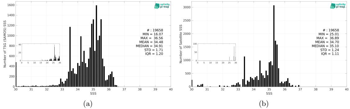
Figure 3: Histograms of SSS from TSG (SAMOS) (a) and Aquarius SSS L3 OR v5 - 7-Day running - Rain mask (NASA-GSFC) (b) considering all match-up pairs per bins of 0.1 over the Equatorial Ocean 10N-10S Pi-MEP region and for the full satellite product period.
