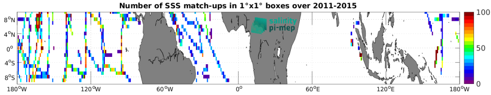
Figure 4: Number of SSS match-ups between TSG (SAMOS) SSS and the Aquarius SSS L3 OR v5 - 7-Day running - Rain mask (NASA-GSFC) SSS product for the Equatorial Ocean 10N-10S Pi-MEP region over 1^\circ \times 1^\circ boxes and for the full satellite product period.
