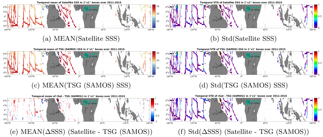
Figure 6: Temporal mean (left) and Std (right) of SSS from Aquarius SSS L3 OR v5 - 7-Day running - Rain mask (NASA-GSFC) (top), TSG (SAMOS) (middle), and of \Delta SSS (Satellite - TSG (SAMOS)). Only match-up pairs are used to generate these maps.
