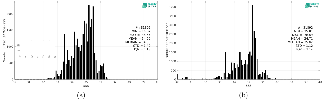
Figure 2: Histograms of SSS from TSG (SAMOS) (a) and Aquarius SSS L3 OR v5 - 7-Day running - Rain mask (NASA-GSFC) (b) considering all match-up pairs per bins of 0.1 over the Equatorial Ocean 10N-10S Pi-MEP region and for the full satellite product period.
