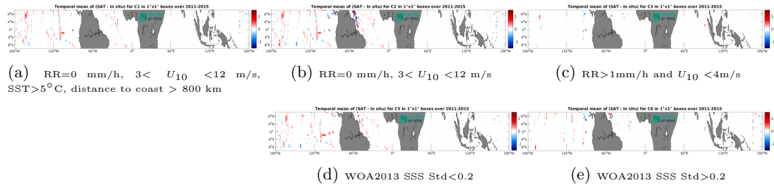
Figure 12: Temporal mean gridded over spatial boxes of size 1^\circ \times 1^\circ of \Delta SSS (Aquarius SSS L3 OR v5 - 7-Day running - Rain mask (NASA-GSFC) - TSG (SAMOS)) for 5 different subdatasets corresponding to:RR=0 mm/h, 3 < U_{10} < 12 m/s, SST >5^\circ C, distance to coast > 800 km (a), RR=0 mm/h, 3 < U_{10} < 12 m/s (b), RR >1 mm/h and U_{10} < 4 m/s (c), WOA2013 SSS Std <0.2 (d), WOA2013 SSS Std >0.2 (e).
