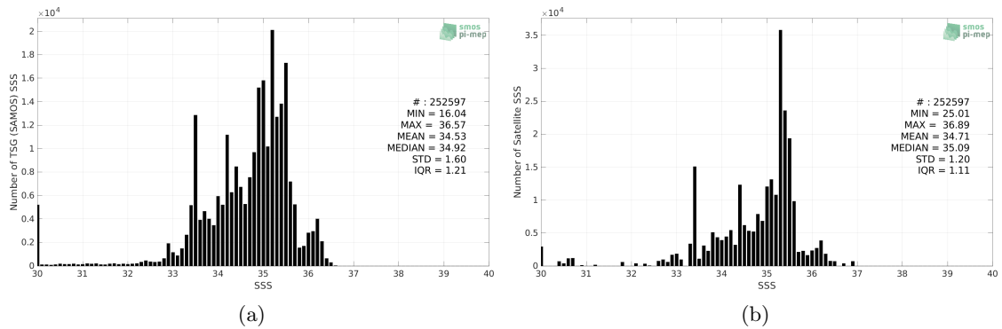
Figure 2: Histograms of SSS from TSG (SAMOS) (a) and Aquarius SSS L3 OR v5 - 7-Day running - Rain mask (NASA-GSFC) (b) considering all match-up pairs per bins of 0.1 over the Equatorial Ocean 10N-10S Pi-MEP region and for the full satellite product period.
