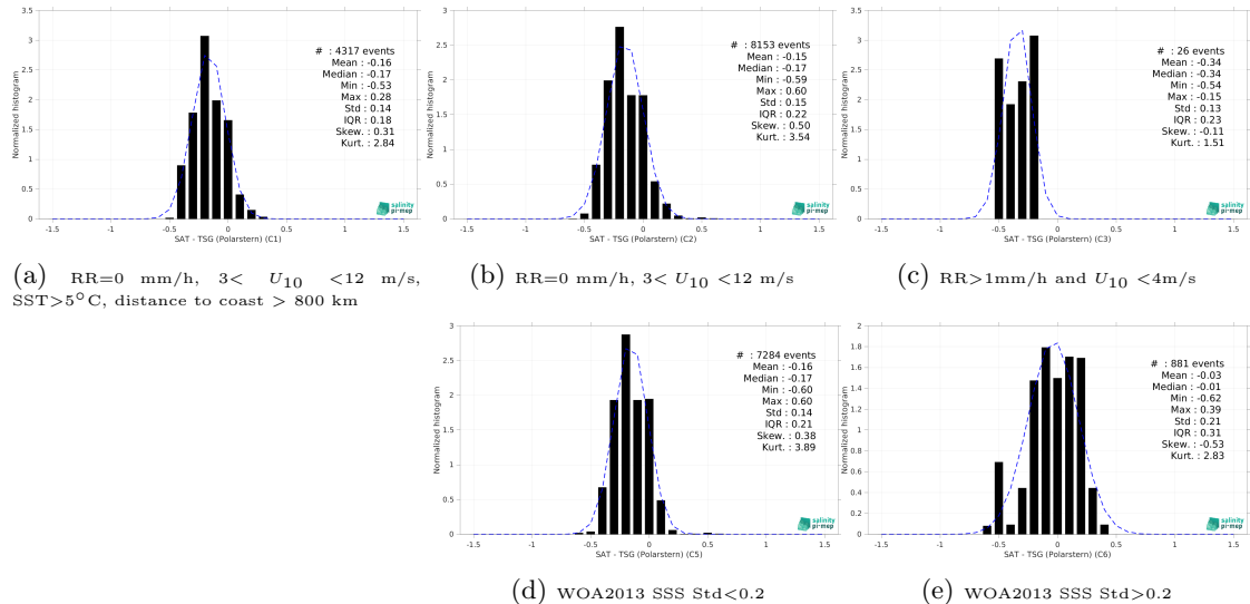
Figure 15: Normalized histogram of \Delta SSS (Aquarius SSS L3 OR v5 - 7-Day running - Rain mask (NASA-GSFC) - TSG (Polarstern)) for 5 different subdatasets corresponding to: RR=0 mm/h, 3 < U_{10} < 12 m/s, SST>5°C, distance to coast > 800 km (a), RR=0 mm/h, 3 < U_{10} < 12 m/s (b), RR>1mm/h and U_{10} < 4 m/s (c), WOA2013 SSS Std<0.2 (d), WOA2013 SSS Std>0.2 (e).
