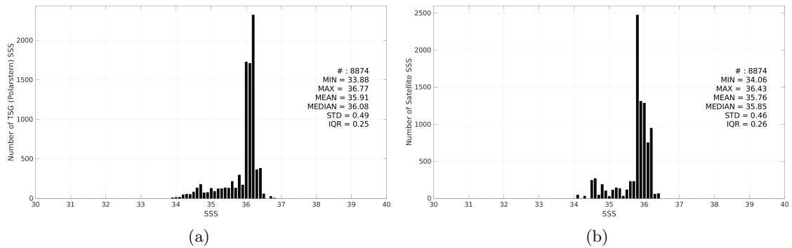
Figure 3: Histograms of SSS from TSG (Polarstern) (a) and Aquarius SSS L3 OR v5 - 7-Day running - Rain mask (NASA-GSFC) (b) considering all match-up pairs per bins of 0.1 over the Equatorial Ocean 10N-10S Pi-MEP region and for the full satellite product period.
