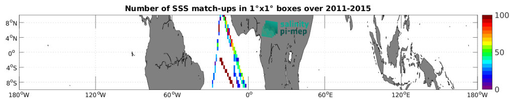
Figure 5: Number of SSS match-ups between TSG (Polarstern) SSS and the Aquarius SSS L3 OR v5 - 7-Day running - Rain mask (NASA-GSFC) SSS product for the Equatorial Ocean 10N-10S Pi-MEP region over 1^\circ \times 1^\circ boxes and for the full satellite product period.
