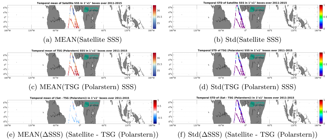
Figure 7: Temporal mean (left) and Std (right) of SSS from Aquarius SSS L3 OR v5 - 7-Day running - Rain mask (NASA-GSFC) (top), TSG (Polarstern) (middle), and of \Delta SSS (Satellite - TSG (Polarstern)). Only match-up pairs are used to generate these maps.
