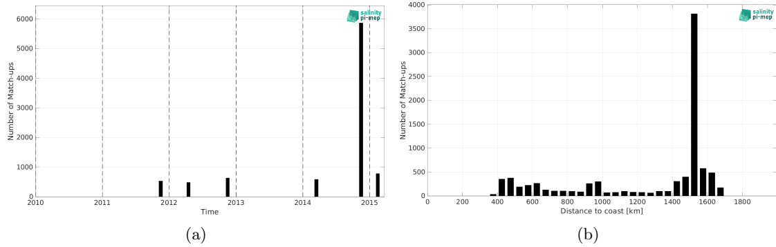
Figure 2: Number of match-ups between TSG (Polarstern) and Aquarius SSS L3 OR v5 - 7-Day running - Rain mask (NASA-GSFC) SSS as a function of time (a) and as function of the distance to coast (b) over the Equatorial Ocean 10N-10S Pi-MEP region and for the full satellite product period.
