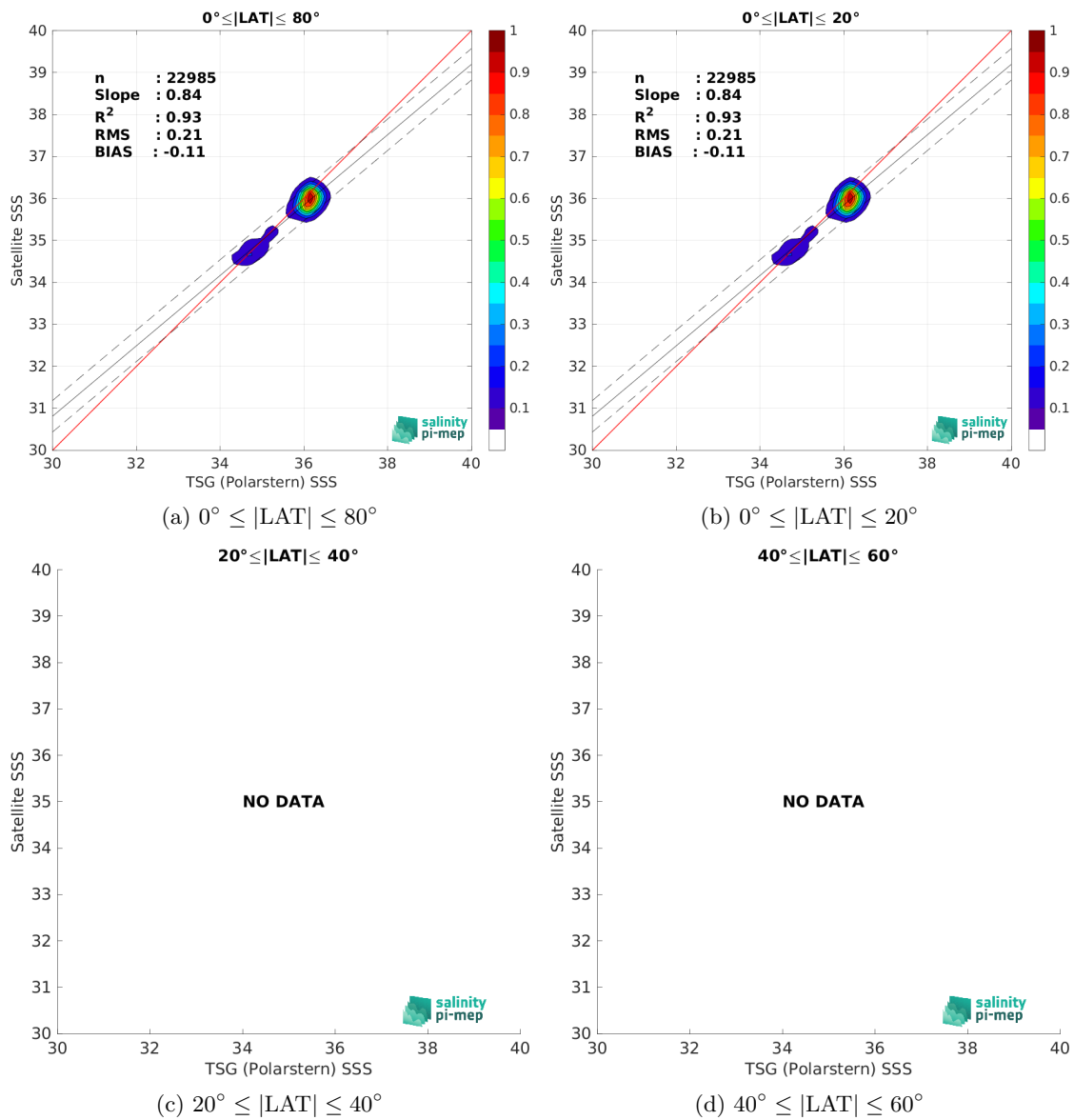
Figure 9: Contour maps of the concentration of Aquarius SSS L3 OR v5 - 7-Day running - Rain mask (NASA-GSFC) SSS (y-axis) versus TSG (Polarstern) SSS (x-axis) at match-up pairs for different latitude bands. For each plot, the red line shows x=y . The black thin and dashed lines indicate a linear fit through the data cloud and the \pm 95\% confidence levels, respectively. The number match-up pairs n , the slope and R^2 coefficient of the linear fit, the root mean square (RMS) and the mean bias between satellite and in situ data are indicated for each latitude band in each plots.
