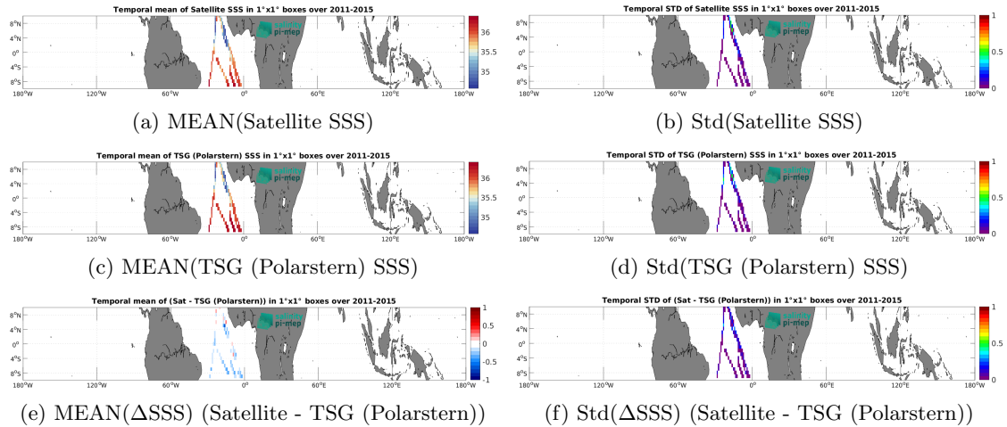
Figure 6: Temporal mean (left) and Std (right) of SSS from Aquarius SSS L3 OR v5 - 7-Day running - Rain mask (NASA-GSFC) (top), TSG (Polarstern) (middle), and of \Delta SSS (Satellite - TSG (Polarstern)). Only match-up pairs are used to generate these maps.
