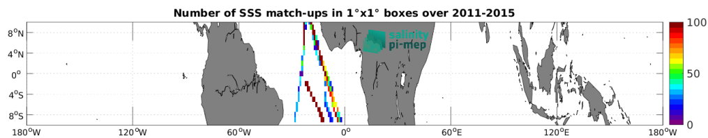
Figure 4: Number of SSS match-ups between TSG (Polarstern) SSS and the Aquarius SSS L3 OR v5 - 7-Day running - Rain mask (NASA-GSFC) SSS product for the Equatorial Ocean 10N-10S Pi-MEP region over 1^\circ \times 1^\circ boxes and for the full satellite product period.
