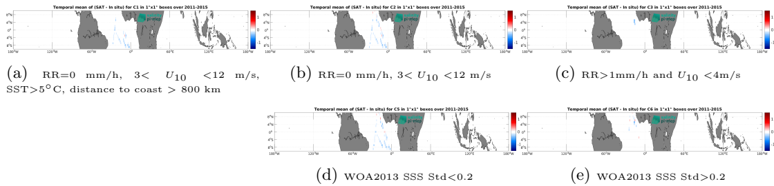
Figure 12: Temporal mean gridded over spatial boxes of size 1^{\circ}\times 1^{\circ} of \Delta\text{SSS} (Aquarius SSS L3 OR v5 - 7-Day running - Rain mask (NASA-GSFC) - TSG (Polarstern)) for 5 different subdatasets corresponding to:RR=0 mm/h, 3 < U_{10} < 12 m/s, SST >5^{\circ}\text{C} , distance to coast > 800 km (a), RR=0 mm/h, 3 < U_{10} < 12 m/s (b), RR >1 mm/h and U_{10} < 4 m/s (c), WOA2013 SSS Std <0.2 (d), WOA2013 SSS Std >0.2 (e).
