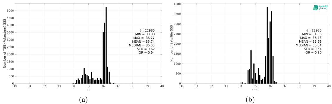
Figure 2: Histograms of SSS from TSG (Polarstern) (a) and Aquarius SSS L3 OR v5 - 7-Day running - Rain mask (NASA-GSFC) (b) considering all match-up pairs per bins of 0.1 over the Equatorial Ocean 10N-10S Pi-MEP region and for the full satellite product period.
