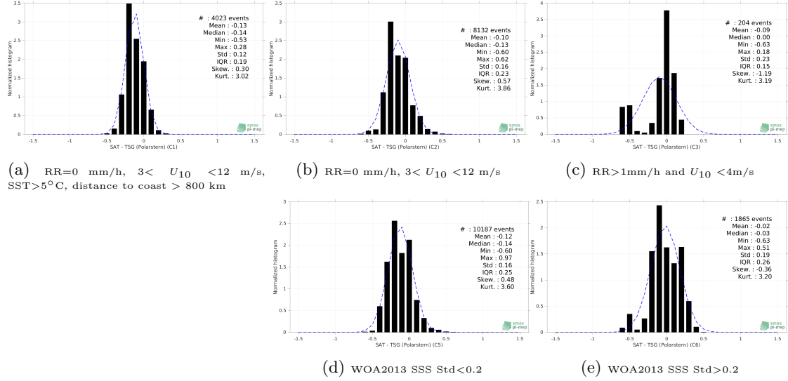
Figure 13: Normalized histogram of \Delta\text{SSS} (Aquarius SSS L3 OR v5 - 7-Day running - Rain mask (NASA-GSFC) - TSG (Polarstern)) for 5 different subdatasets corresponding to: RR=0 mm/h, 3 < U_{10} < 12 m/s, SST>5°C, distance to coast > 800 km (a), RR=0 mm/h, 3 < U_{10} < 12 m/s (b), RR>1mm/h and U_{10} < 4 m/s (c), WOA2013 SSS Std<0.2 (d), WOA2013 SSS Std>0.2 (e).
