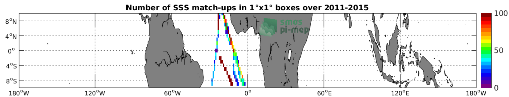
Figure 4: Number of SSS match-ups between TSG-POLARSTERN SSS and the Aquarius-L3-OR-V5-7DAY-RUNNING-RAIN-MASK-1DEG SSS product for the Equatorial Ocean 10N-10S Pi-MEP region over 1^\circ \times 1^\circ boxes and for the full satellite product period.
