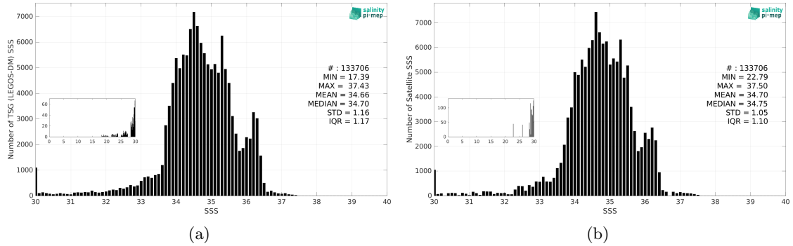
Figure 3: Histograms of SSS from TSG (LEGOS-DM) (a) and Aquarius SSS L3 OR v5 - 7-Day running - Rain mask (NASA-GSFC) (b) considering all match-up pairs per bins of 0.1 over the Equatorial Ocean 10N-10S Pi-MEP region and for the full satellite product period.
