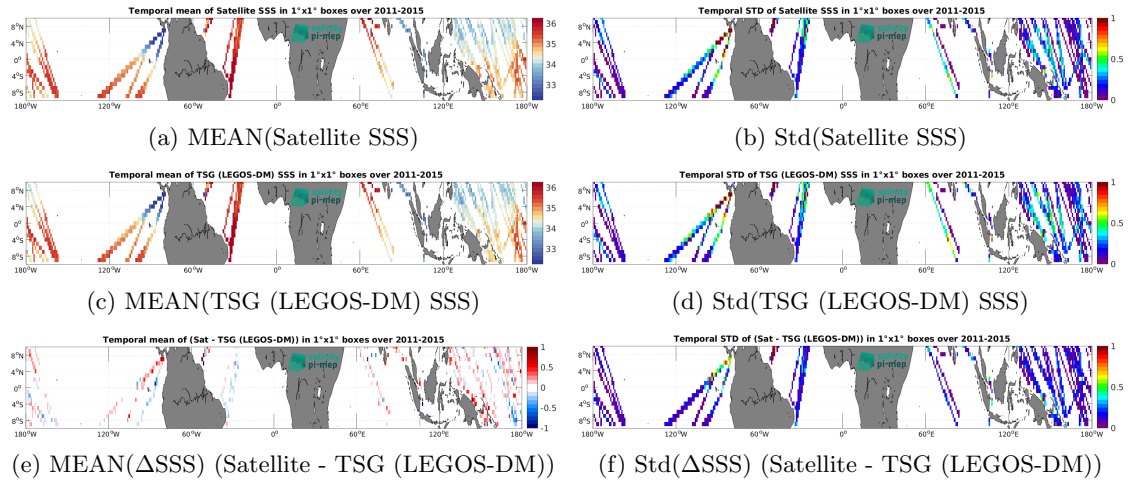
Figure 7: Temporal mean (left) and Std (right) of SSS from Aquarius SSS L3 OR v5 - 7-Day running - Rain mask (NASA-GSFC) (top), TSG (LEGOS-DM) (middle), and of \Delta SSS (Satellite - TSG (LEGOS-DM)). Only match-up pairs are used to generate these maps.
