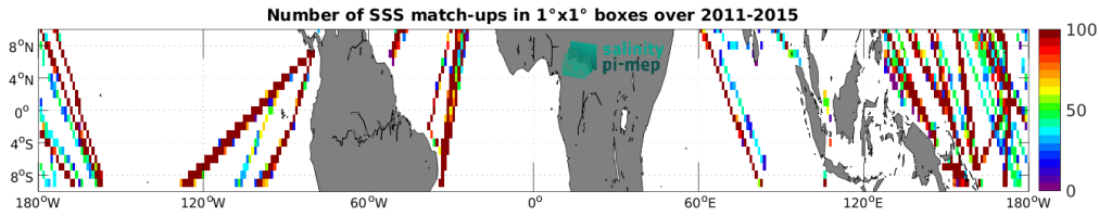
Figure 5: Number of SSS match-ups between TSG (LEGOS-DM) SSS and the Aquarius SSS L3 OR v5 - 7-Day running - Rain mask (NASA-GSFC) SSS product for the Equatorial Ocean 10N-10S Pi-MEP region over 1^\circ \times 1^\circ boxes and for the full satellite product period.
