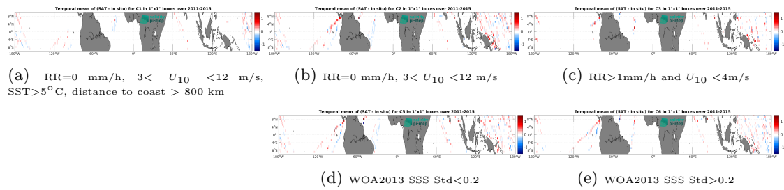
Figure 14: Temporal mean gridded over spatial boxes of size 1^\circ \times 1^\circ of \Delta SSS (Aquarius SSS L3 OR v5 - 7-Day running - Rain mask (NASA-GSFC) - TSG (LEGOS-DM)) for 5 different subdatasets corresponding to:RR=0 mm/h, 3 < U_{10} < 12 m/s, SST >5^\circ C, distance to coast > 800 km (a), RR=0 mm/h, 3 < U_{10} < 12 m/s (b), RR >1 mm/h and U_{10} < 4 m/s (c), WOA2013 SSS Std <0.2 (d), WOA2013 SSS Std >0.2 (e).
