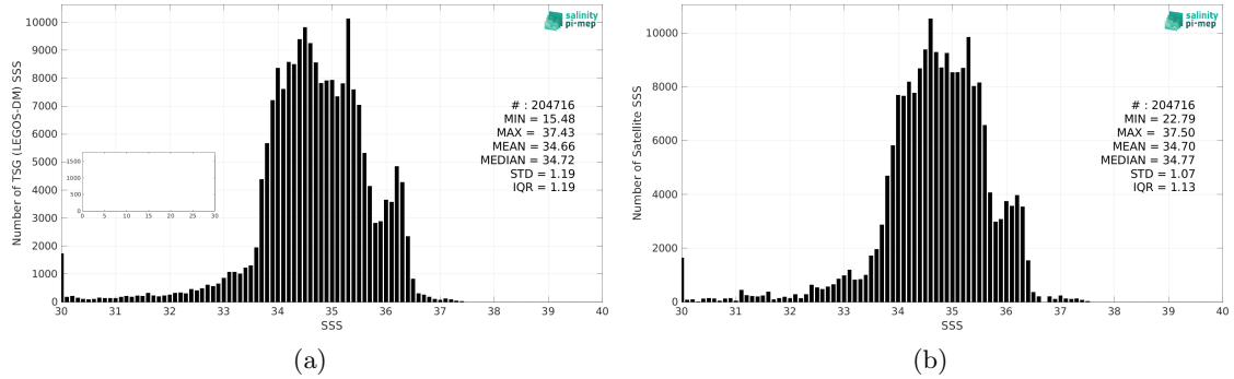
Figure 2: Histograms of SSS from TSG (LEGOS-DM) (a) and Aquarius SSS L3 OR v5 - 7-Day running - Rain mask (NASA-GSFC) (b) considering all match-up pairs per bins of 0.1 over the Equatorial Ocean 10N-10S Pi-MEP region and for the full satellite product period.
