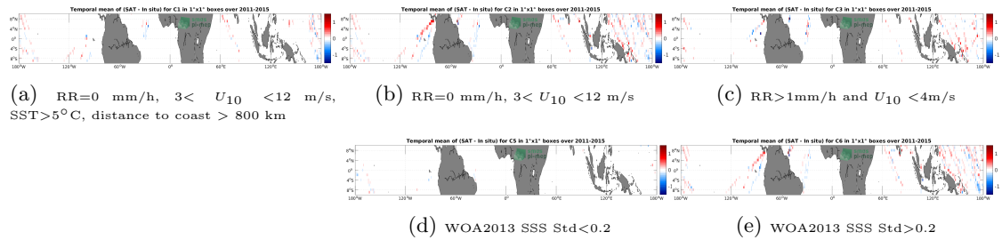
Figure 12: Temporal mean gridded over spatial boxes of size 1^{\circ}\times 1^{\circ} of \Delta\text{SSS} (Aquarius SSS L3 OR v5 - 7-Day running - Rain mask (NASA-GSFC) - TSG (LEGOS-DM)) for 5 different subdatasets corresponding to:RR=0 mm/h, 3 < U_{10} < 12 m/s, SST >5^{\circ}\text{C} , distance to coast > 800 km (a), RR=0 mm/h, 3 < U_{10} < 12 m/s (b), RR >1 mm/h and U_{10} < 4 m/s (c), WOA2013 SSS Std <0.2 (d), WOA2013 SSS Std >0.2 (e).
