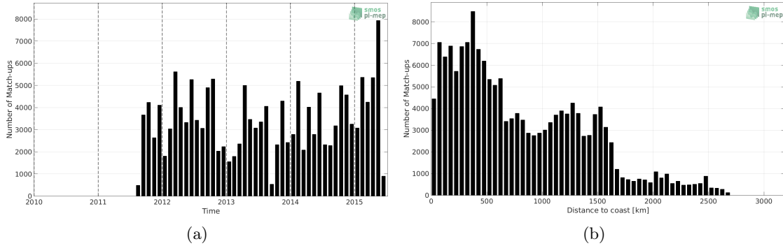
Figure 1: Number of match-ups between TSG-LEGOS-DM and Aquarius-L3-OR-V5-7DAY-RUNNING-RAIN-MASK-1DEG SSS as a function of time (a) and as function of the distance to coast (b) over the Equatorial Ocean 10N-10S Pi-MEP region and for the full satellite product period.
