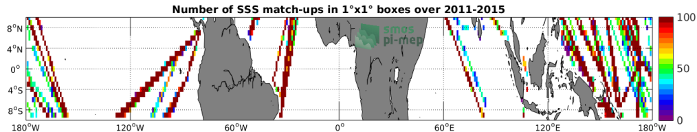
Figure 4: Number of SSS match-ups between TSG-LEGOS-DM SSS and the Aquarius-L3-OR-V5-7DAY-RUNNING-RAIN-MASK-1DEG SSS product for the Equatorial Ocean 10N-10S Pi-MEP region over 1°x1° boxes and for the full satellite product period.
