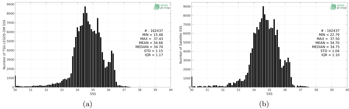
Figure 2: Histograms of SSS from TSG-LEGOS-DM (a) and Aquarius-L3-OR-V5-7DAY-RUNNING-RAIN-MASK-1DEG (b) considering all match-up pairs per bins of 0.1 over the Equatorial Ocean 10N-10S Pi-MEP region and for the full satellite product period.
