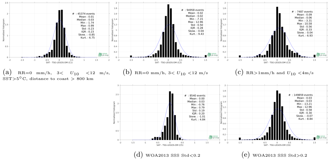
Figure 13: Normalized histogram of \Delta SSS (Aquarius-L3-OR-V5-7DAY-RUNNING-RAIN-MASK-1DEG - TSG-LEGOS-DM) for 5 different subdatasets corresponding to: RR=0 mm/h, 3 < U_{10} < 12 m/s, SST >5^\circ\text{C} , distance to coast > 800 km (a), RR=0 mm/h, 3 < U_{10} < 12 m/s (b), RR >1 mm/h and U_{10} < 4 m/s (c), WOA2013 SSS Std <0.2 (d), WOA2013 SSS Std >0.2 (e).
