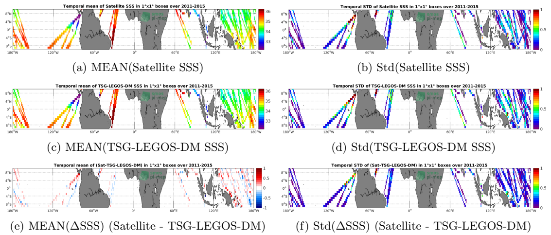
Figure 6: Temporal mean (left) and Std (right) of SSS from Aquarius-L3-OR-V5-7DAY-RUNNING-RAIN-MASK-1DEG (top), TSG-LEGOS-DM (middle), and of \Delta SSS (Satellite - TSG-LEGOS-DM). Only match-up pairs are used to generate these maps.
