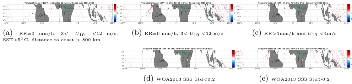
Figure 12: Temporal mean gridded over spatial boxes of size 1^\circ \times 1^\circ of \Delta SSS (Aquarius-L3-OR-V5-7DAY-RUNNING-RAIN-MASK-1DEG - TSG-LEGOS-DM) for 5 different subdatasets corresponding to: RR=0 mm/h, 3 < U_{10} < 12 m/s, SST >5^\circ\text{C} , distance to coast > 800 km (a), RR=0 mm/h, 3 < U_{10} < 12 m/s (b), RR >1 mm/h and U_{10} < 4 m/s (c), WOA2013 SSS Std <0.2 (d), WOA2013 SSS Std >0.2 (e).
