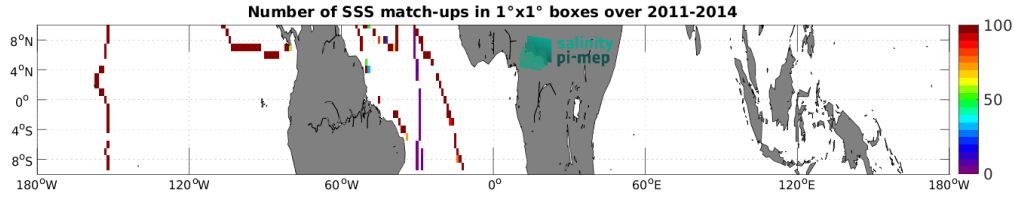
Figure 5: Number of SSS match-ups between TSG (GOSUD-Sailing-ship) SSS and the Aquarius SSS L3 OR v5 - 7-Day running - Rain mask (NASA-GSFC) SSS product for the Equatorial Ocean 10N-10S Pi-MEP region over 1^\circ \times 1^\circ boxes and for the full satellite product period.
