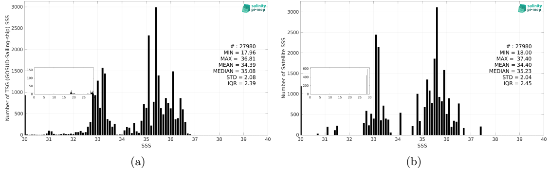
Figure 3: Histograms of SSS from TSG (GOSUD-Sailing-ship) (a) and Aquarius SSS L3 OR v5 - 7-Day running - Rain mask (NASA-GSFC) (b) considering all match-up pairs per bins of 0.1 over the Equatorial Ocean 10N-10S Pi-MEP region and for the full satellite product period.
