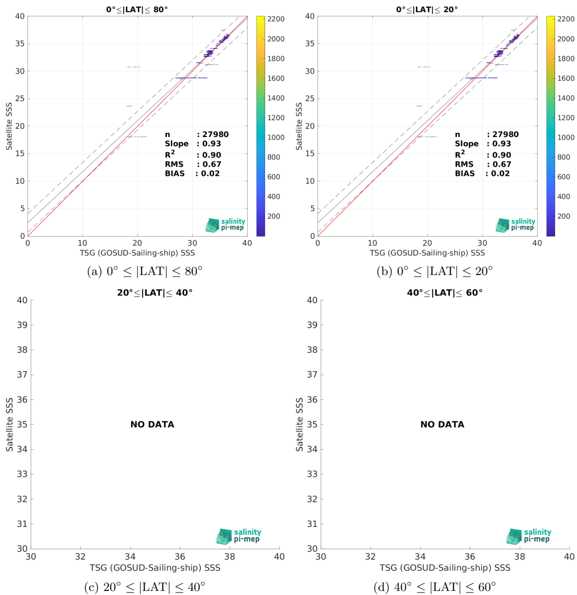
Figure 10: Contour maps of the concentration of Aquarius SSS L3 OR v5 - 7-Day running - Rain mask (NASA-GSFC) SSS (y-axis) versus TSG (GOSUD-Sailing-ship) SSS (x-axis) at match-up pairs for different latitude bands. For each plot, the red line shows x=y . The black thin and dashed lines indicate a linear fit through the data cloud and the \pm 95\% confidence levels, respectively. The number match-up pairs n , the slope and R^2 coefficient of the linear fit, the root mean square (RMS) and the mean bias between satellite and in situ data are indicated for each latitude band in each plots.
