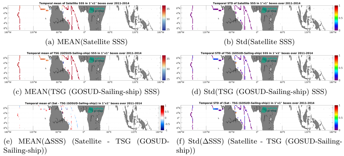
Figure 7: Temporal mean (left) and Std (right) of SSS from Aquarius SSS L3 OR v5 - 7-Day running - Rain mask (NASA-GSFC) (top), TSG (GOSUD-Sailing-ship) (middle), and of \Delta SSS (Satellite - TSG (GOSUD-Sailing-ship)). Only match-up pairs are used to generate these maps.
