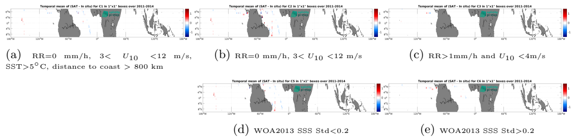
Figure 14: Temporal mean gridded over spatial boxes of size 1^\circ \times 1^\circ of \Delta SSS (Aquarius SSS L3 OR v5 - 7-Day running - Rain mask (NASA-GSFC) - TSG (GOSUD-Sailing-ship)) for 5 different subdatasets corresponding to:RR=0 mm/h, 3 < U_{10} < 12 m/s, SST >5^\circ C, distance to coast > 800 km (a), RR=0 mm/h, 3 < U_{10} < 12 m/s (b), RR >1 mm/h and U_{10} < 4 m/s (c), WOA2013 SSS Std <0.2 (d), WOA2013 SSS Std >0.2 (e).
