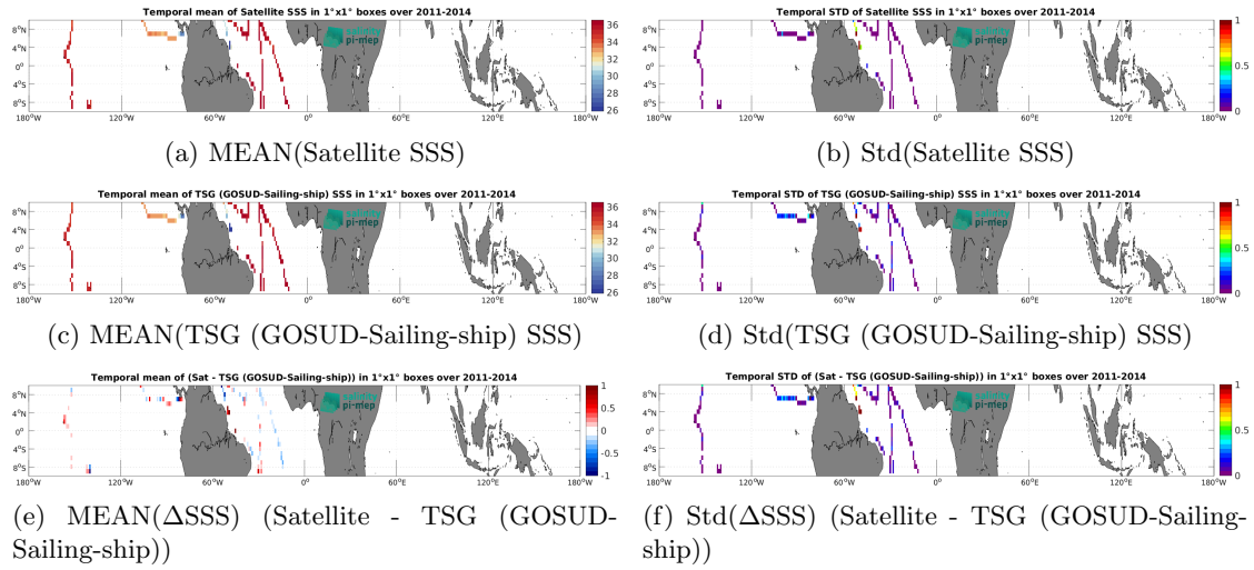
Figure 6: Temporal mean (left) and Std (right) of SSS from Aquarius SSS L3 OR v5 - 7-Day running - Rain mask (NASA-GSFC) (top), TSG (GOSUD-Sailing-ship) (middle), and of \Delta SSS (Satellite - TSG (GOSUD-Sailing-ship)). Only match-up pairs are used to generate these maps.
