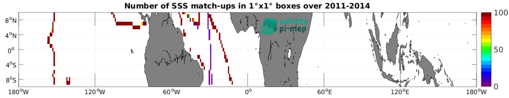
Figure 4: Number of SSS match-ups between TSG (GOSUD-Sailing-ship) SSS and the Aquarius SSS L3 OR v5 - 7-Day running - Rain mask (NASA-GSFC) SSS product for the Equatorial Ocean 10N-10S Pi-MEP region over 1^\circ \times 1^\circ boxes and for the full satellite product period.
