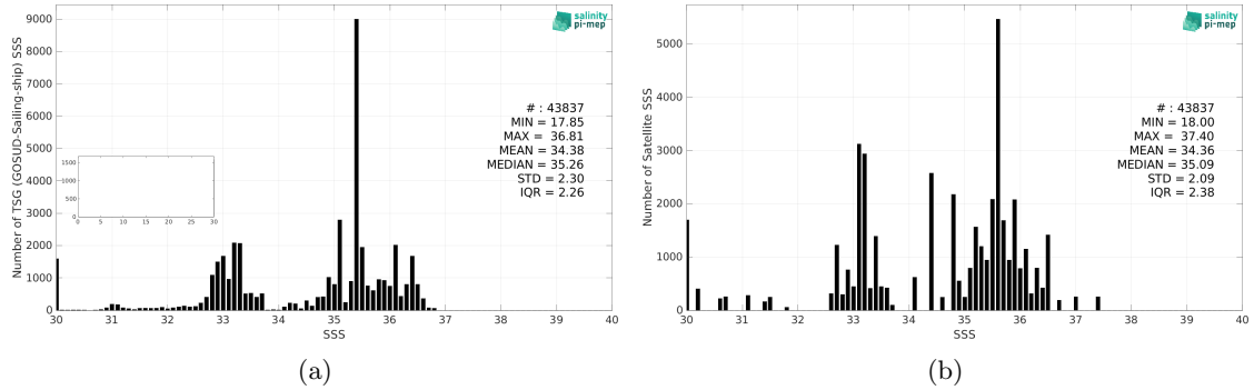
Figure 2: Histograms of SSS from TSG (GOSUD-Sailing-ship) (a) and Aquarius SSS L3 OR v5 - 7-Day running - Rain mask (NASA-GSFC) (b) considering all match-up pairs per bins of 0.1 over the Equatorial Ocean 10N-10S Pi-MEP region and for the full satellite product period.
