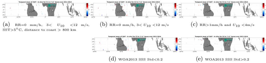
Figure 12: Temporal mean gridded over spatial boxes of size 1^{\circ}\times 1^{\circ} of \Delta SSS (Aquarius SSS L3 OR v5 - 7-Day running - Rain mask (NASA-GSFC) - TSG (GOSUD-Sailing-ship)) for 5 different subdatasets corresponding to:RR=0 mm/h, 3 < U_{10} < 12 m/s, SST > 5^{\circ}\text{C} , distance to coast > 800 km (a), RR=0 mm/h, 3 < U_{10} < 12 m/s (b), RR > 1 mm/h and U_{10} < 4 m/s (c), WOA2013 SSS Std < 0.2 (d), WOA2013 SSS Std > 0.2 (e).
