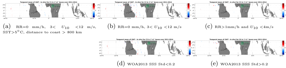
Figure 12: Temporal mean gridded over spatial boxes of size 1^\circ \times 1^\circ of \Delta SSS (Aquarius SSS L3 OR v5 - 7-Day running - Rain mask (NASA-GSFC) - TSG (GOSUD-Sailing-ship)) for 5 different subdatasets corresponding to:RR=0 mm/h, 3 < U_{10} < 12 m/s, SST >5^\circ\text{C} , distance to coast > 800 km (a), RR=0 mm/h, 3 < U_{10} < 12 m/s (b), RR >1 mm/h and U_{10} < 4 m/s (c), WOA2013 SSS Std <0.2 (d), WOA2013 SSS Std >0.2 (e).
