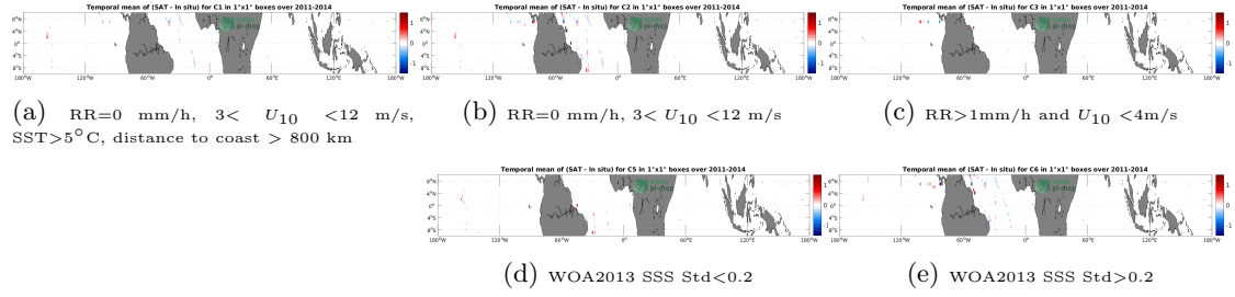
Figure 12: Temporal mean gridded over spatial boxes of size 1^{\circ}\times 1^{\circ} of \Delta SSS (Aquarius SSS L3 OR v5 - 7-Day running - Rain mask (NASA-GSFC) - TSG (GOSUD-Sailing-ship)) for 5 different subdatasets corresponding to:RR=0 mm/h, 3 < U_{10} < 12 m/s, SST >5^{\circ}\text{C} , distance to coast > 800 km (a), RR=0 mm/h, 3 < U_{10} < 12 m/s (b), RR >1 mm/h and U_{10} < 4 m/s (c), WOA2013 SSS Std <0.2 (d), WOA2013 SSS Std >0.2 (e).
