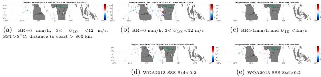
Figure 12: Temporal mean gridded over spatial boxes of size 1^\circ \times 1^\circ of \Delta SSS (Aquarius SSS L3 OR v5 - 7-Day running - Rain mask (NASA-GSFC) - TSG (GOSUD-Research-vessel)) for 5 different subdatasets corresponding to:RR=0 mm/h, 3 < U_{10} < 12 m/s, SST >5^\circ\text{C} , distance to coast > 800 km (a), RR=0 mm/h, 3 < U_{10} < 12 m/s (b), RR >1 mm/h and U_{10} < 4 m/s (c), WOA2013 SSS Std <0.2 (d), WOA2013 SSS Std >0.2 (e).
