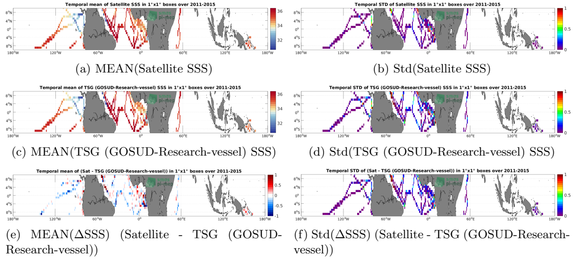
Figure 6: Temporal mean (left) and Std (right) of SSS from Aquarius SSS L3 OR v5 - 7-Day running - Rain mask (NASA-GSFC) (top), TSG (GOSUD-Research-vessel) (middle), and of \Delta SSS (Satellite - TSG (GOSUD-Research-vessel)). Only match-up pairs are used to generate these maps.
