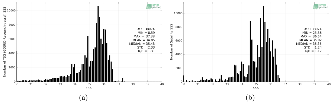
Figure 2: Histograms of SSS from TSG (GOSUD-Research-vessel) (a) and Aquarius SSS L3 OR v5 - 7-Day running - Rain mask (NASA-GSFC) (b) considering all match-up pairs per bins of 0.1 over the Equatorial Ocean 10N-10S Pi-MEP region and for the full satellite product period.
