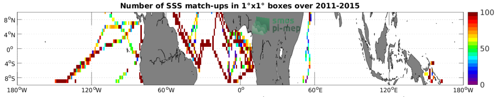
Figure 4: Number of SSS match-ups between TSG (GOSUD-Research-vessel) SSS and the Aquarius SSS L3 OR v5 - 7-Day running - Rain mask (NASA-GSFC) SSS product for the Equatorial Ocean 10N-10S Pi-MEP region over 1^\circ \times 1^\circ boxes and for the full satellite product period.
