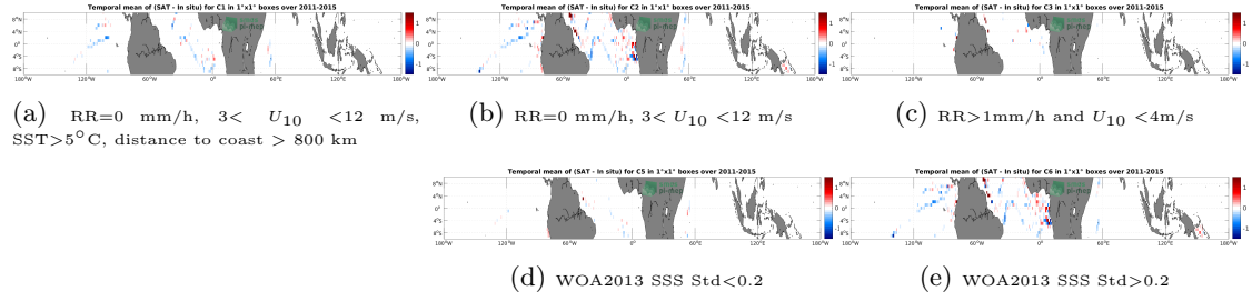
Figure 12: Temporal mean gridded over spatial boxes of size 1^{\circ}\times 1^{\circ} of \Delta SSS (Aquarius SSS L3 OR v5 - 7-Day running - Rain mask (NASA-GSFC) - TSG (GOSUD-Research-vessel)) for 5 different subdatasets corresponding to:RR=0 mm/h, 3 < U_{10} < 12 m/s, SST >5^{\circ}\text{C} , distance to coast > 800 km (a), RR=0 mm/h, 3 < U_{10} < 12 m/s (b), RR >1 mm/h and U_{10} < 4 m/s (c), WOA2013 SSS Std <0.2 (d), WOA2013 SSS Std >0.2 (e).
