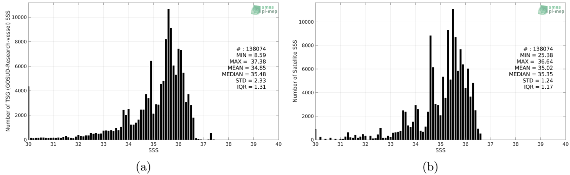
Figure 2: Histograms of SSS from TSG (GOSUD-Research-vessel) (a) and Aquarius SSS L3 OR v5 - 7-Day running - Rain mask (NASA-GSFC) (b) considering all match-up pairs per bins of 0.1 over the Equatorial Ocean 10N-10S Pi-MEP region and for the full satellite product period.
