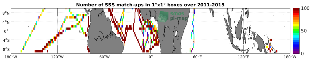
Figure 4: Number of SSS match-ups between TSG-GOSUD-Research-vessel SSS and the Aquarius-L3-OR-V5-7DAY-RUNNING-RAIN-MASK-1DEG SSS product for the Equatorial Ocean 10N-10S Pi-MEP region over 1^\circ \times 1^\circ boxes and for the full satellite product period.
