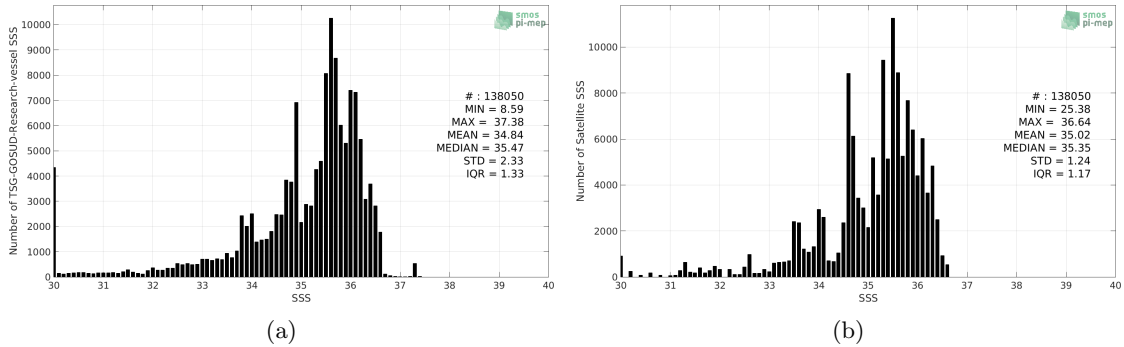
Figure 2: Histograms of SSS from TSG-GOSUD-Research-vessel (a) and Aquarius-L3-OR-V5-7DAY-RUNNING-RAIN-MASK-1DEG (b) considering all match-up pairs per bins of 0.1 over the Equatorial Ocean 10N-10S Pi-MEP region and for the full satellite product period.
