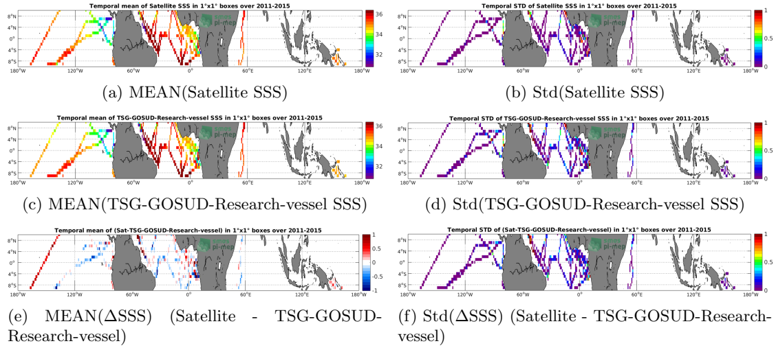
Figure 6: Temporal mean (left) and Std (right) of SSS from Aquarius-L3-OR-V5-7DAY-RUNNING-RAIN-MASK-1DEG (top), TSG-GOSUD-Research-vessel (middle), and of \Delta SSS (Satellite - TSG-GOSUD-Research-vessel). Only match-up pairs are used to generate these maps.
