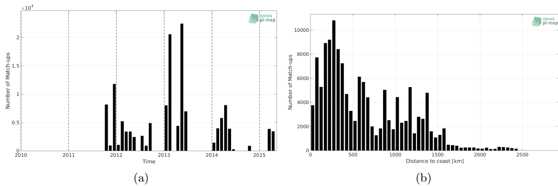
Figure 1: Number of match-ups between TSG-GOSUD-Research-vessel and Aquarius-L3-OR-V5-7DAY-RUNNING-RAIN-MASK-1DEG SSS as a function of time (a) and as function of the distance to coast (b) over the Equatorial Ocean 10N-10S Pi-MEP region and for the full satellite product period.
