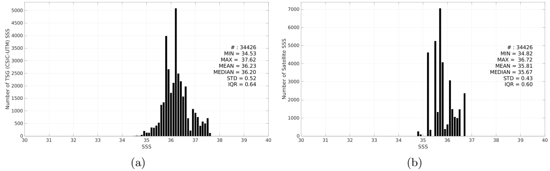
Figure 3: Histograms of SSS from TSG (CSIC-UTM) (a) and Aquarius SSS L3 OR v5 - 7-Day running - Rain mask (NASA-GSFC) (b) considering all match-up pairs per bins of 0.1 over the Equatorial Ocean 10N-10S Pi-MEP region and for the full satellite product period.
