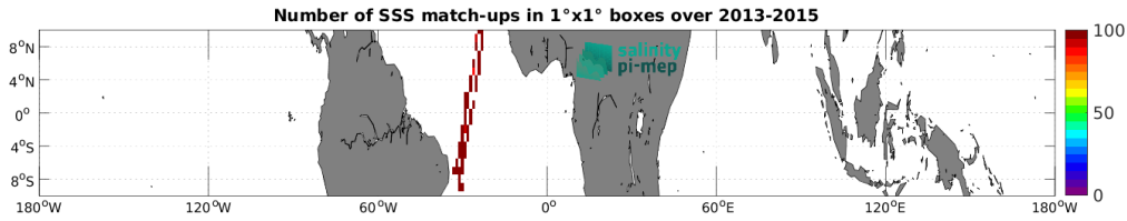
Figure 5: Number of SSS match-ups between TSG (CSIC-UTM) SSS and the Aquarius SSS L3 OR v5 - 7-Day running - Rain mask (NASA-GSFC) SSS product for the Equatorial Ocean 10N-10S Pi-MEP region over 1^\circ \times 1^\circ boxes and for the full satellite product period.
