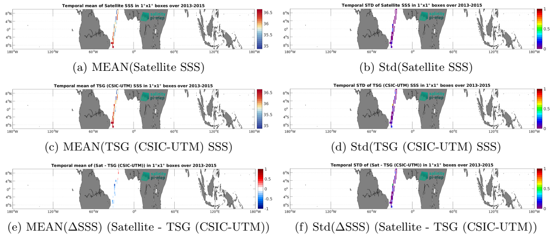
Figure 7: Temporal mean (left) and Std (right) of SSS from Aquarius SSS L3 OR v5 - 7-Day running - Rain mask (NASA-GSFC) (top), TSG (CSIC-UTM) (middle), and of \Delta SSS (Satellite - TSG (CSIC-UTM)). Only match-up pairs are used to generate these maps.
