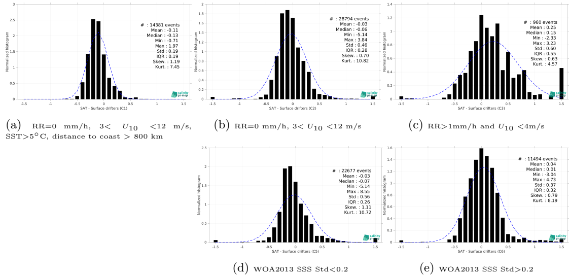
Figure 14: Normalized histogram of \Delta SSS (Aquarius SSS L3 OR v5 - 7-Day running - Rain mask (NASA-GSFC) - Surface drifters) for 5 different subdatasets corresponding to: RR=0 mm/h, 3 < U_{10} < 12 m/s, SST >5^\circ\text{C} , distance to coast > 800 km (a), RR=0 mm/h, 3 < U_{10} < 12 m/s (b), RR >1 mm/h and U_{10} < 4 m/s (c), WOA2013 SSS Std <0.2 (d), WOA2013 SSS Std >0.2 (e).
