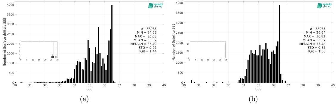
Figure 3: Histograms of SSS from Surface drifters (a) and Aquarius SSS L3 OR v5 - 7-Day running - Rain mask (NASA-GSFC) (b) considering all match-up pairs per bins of 0.1 over the Equatorial Ocean 10N-10S Pi-MEP region and for the full satellite product period.
