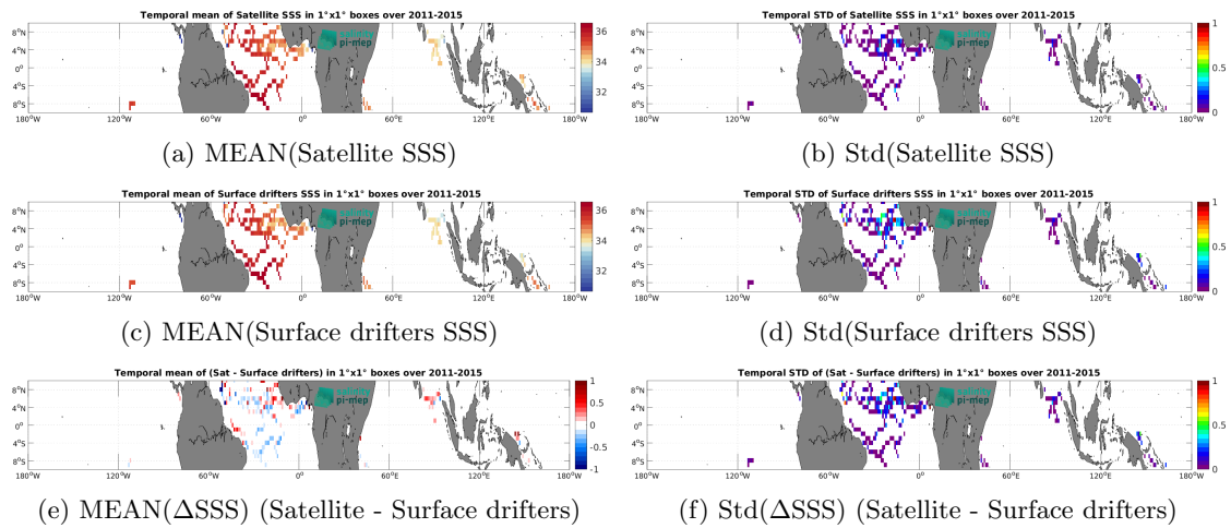
Figure 6: Temporal mean (left) and Std (right) of SSS from Aquarius SSS L3 OR v5 - 7-Day running - Rain mask (NASA-GSFC) (top), Surface drifters (middle), and of \Delta SSS (Satellite - Surface drifters). Only match-up pairs are used to generate these maps.
