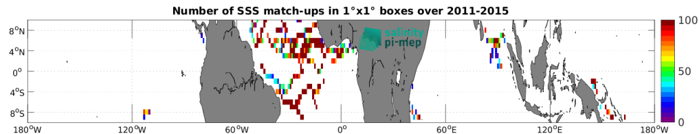
Figure 4: Number of SSS match-ups between Surface drifters SSS and the Aquarius SSS L3 OR v5 - 7-Day running - Rain mask (NASA-GSFC) SSS product for the Equatorial Ocean 10N-10S Pi-MEP region over 1^\circ \times 1^\circ boxes and for the full satellite product period.
