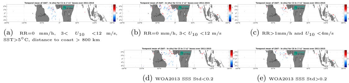
Figure 11: Temporal mean gridded over spatial boxes of size 1^\circ \times 1^\circ of \Delta SSS (Aquarius SSS L3 OR v5 - 7-Day running - Rain mask (NASA-GSFC) - Surface drifters) for 5 different subdatasets corresponding to:RR=0 mm/h, 3 < U_{10} < 12 m/s, SST >5^\circ C, distance to coast > 800 km (a), RR=0 mm/h, 3 < U_{10} < 12 m/s (b), RR >1 mm/h and U_{10} < 4 m/s (c), WOA2013 SSS Std <0.2 (d), WOA2013 SSS Std >0.2 (e).
