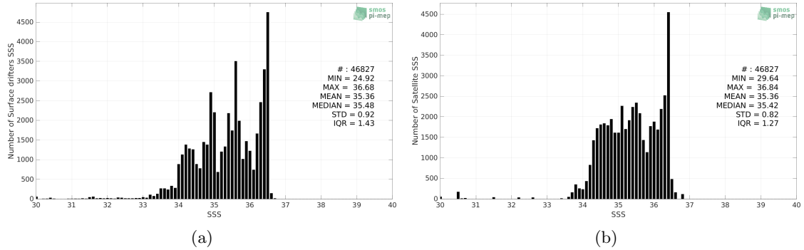
Figure 2: Histograms of SSS from Surface drifters (a) and Aquarius SSS L3 OR v5 - 7-Day running - Rain mask (NASA-GSFC) (b) considering all match-up pairs per bins of 0.1 over the Equatorial Ocean 10N-10S Pi-MEP region and for the full satellite product period.
