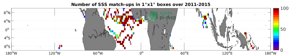
Figure 3: Number of SSS match-ups between Surface drifters SSS and the Aquarius SSS L3 OR v5 - 7-Day running - Rain mask (NASA-GSFC) SSS product for the Equatorial Ocean 10N-10S Pi-MEP region over 1^\circ \times 1^\circ boxes and for the full satellite product period.
