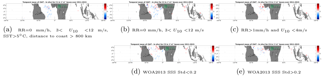
Figure 11: Temporal mean gridded over spatial boxes of size 1^{\circ}\times 1^{\circ} of \Delta\text{SSS} (Aquarius SSS L3 OR v5 - 7-Day running - Rain mask (NASA-GSFC) - Surface drifters) for 5 different subdatasets corresponding to:RR=0 mm/h, 3 < U_{10} < 12 m/s, SST >5^{\circ}\text{C} , distance to coast > 800 km (a), RR=0 mm/h, 3 < U_{10} < 12 m/s (b), RR >1 mm/h and U_{10} < 4 m/s (c), WOA2013 SSS Std <0.2 (d), WOA2013 SSS Std >0.2 (e).
