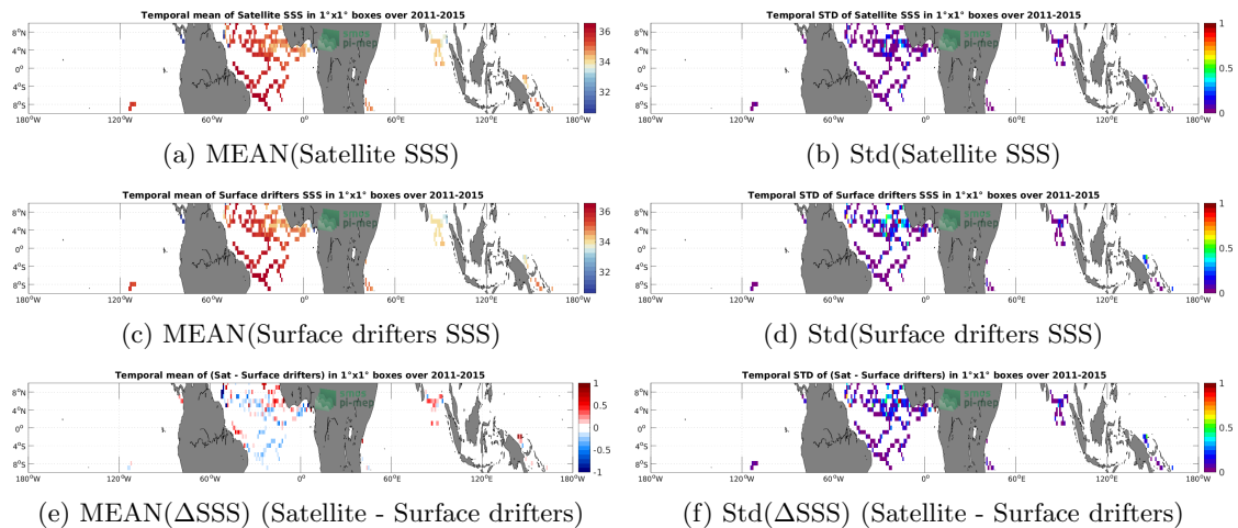
Figure 5: Temporal mean (left) and Std (right) of SSS from Aquarius SSS L3 OR v5 - 7-Day running - Rain mask (NASA-GSFC) (top), Surface drifters (middle), and of \Delta SSS (Satellite - Surface drifters). Only match-up pairs are used to generate these maps.
