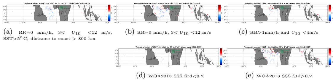
Figure 11: Temporal mean gridded over spatial boxes of size 1^\circ \times 1^\circ of \Delta SSS (Aquarius-L3-OR-V5-7DAY-RUNNING-RAIN-MASK-1DEG - Surface drifters) for 5 different subdatasets corresponding to:RR=0 mm/h, 3 < U_{10} < 12 m/s, SST >5^\circ C, distance to coast > 800 km (a), RR=0 mm/h, 3 < U_{10} < 12 m/s (b), RR >1 mm/h and U_{10} < 4 m/s (c), WOA2013 SSS Std <0.2 (d), WOA2013 SSS Std >0.2 (e).
