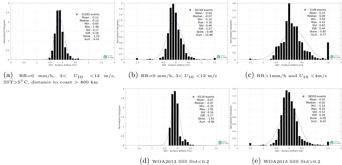
Figure 12: Normalized histogram of \Delta SSS (Aquarius-L3-OR-V5-7DAY-RUNNING-RAIN-MASK-1DEG - Surface drifters) for 5 different subdatasets corresponding to: RR=0 mm/h, 3 < U_{10} < 12 m/s, SST >5^\circ C, distance to coast > 800 km (a), RR=0 mm/h, 3 < U_{10} < 12 m/s (b), RR >1 mm/h and U_{10} < 4 m/s (c), WOA2013 SSS Std <0.2 (d), WOA2013 SSS Std >0.2 (e).
