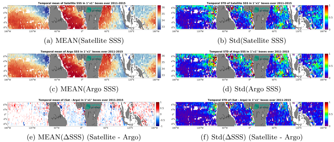
Figure 7: Temporal mean (left) and Std (right) of SSS from Aquarius SSS L3 OR v5 - 7-Day running - Rain mask (NASA-GSFC) (top), Argo (middle), and of \Delta SSS (Satellite - Argo). Only match-up pairs are used to generate these maps.
