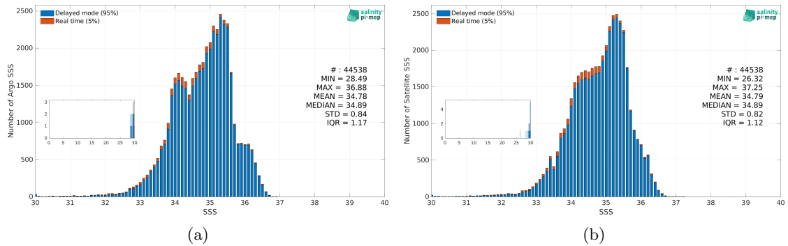
Figure 3: Histograms of SSS from Argo (a) and Aquarius SSS L3 OR v5 - 7-Day running - Rain mask (NASA-GSFC) (b) considering all match-up pairs per bins of 0.1 over the Equatorial Ocean 10N-10S Pi-MEP region and for the full satellite product period.
