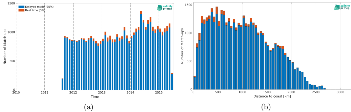
Figure 2: Number of match-ups between Argo and Aquarius SSS L3 OR v5 - 7-Day running - Rain mask (NASA-GSFC) SSS as a function of time (a) and as function of the distance to coast (b) over the Equatorial Ocean 10N-10S Pi-MEP region and for the full satellite product period.
