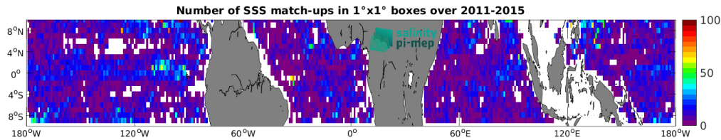
Figure 5: Number of SSS match-ups between Argo SSS and the Aquarius SSS L3 OR v5 - 7-Day running - Rain mask (NASA-GSFC) SSS product for the Equatorial Ocean 10N-10S Pi-MEP region over 1^\circ \times 1^\circ boxes and for the full satellite product period.
