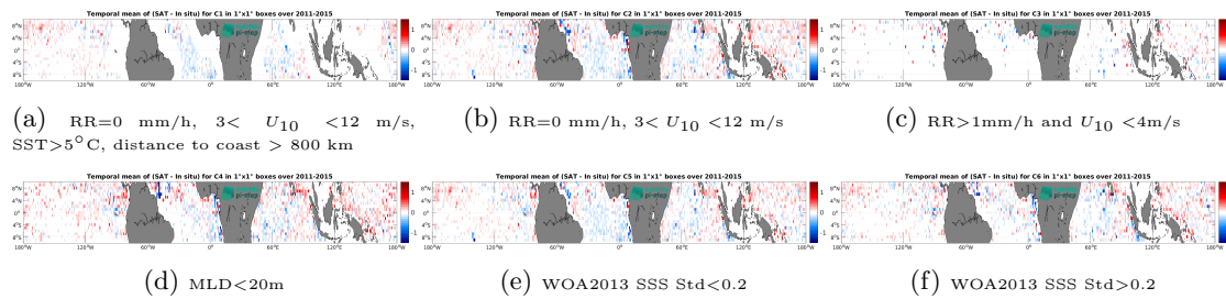
Figure 14: Temporal mean gridded over spatial boxes of size 1^\circ \times 1^\circ of \Delta SSS (Aquarius SSS L3 OR v5 - 7-Day running - Rain mask (NASA-GSFC) - Argo) for 6 different subdatasets corresponding to:RR=0 mm/h, 3 < U_{10} < 12 m/s, SST >5^\circ\text{C} , distance to coast > 800 km (a), RR=0 mm/h, 3 < U_{10} < 12 m/s (b), RR >1 mm/h and U_{10} < 4 m/s (c),MLD <20 m (d),WOA2013 SSS Std <0.2 (e),WOA2013 SSS Std >0.2 (f).
