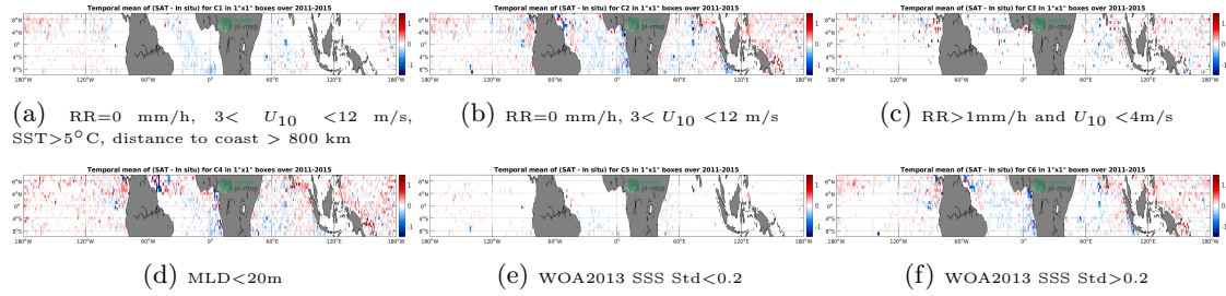
Figure 12: Temporal mean gridded over spatial boxes of size 1^{\circ} \times 1^{\circ} of \Delta\text{SSS} (Aquarius SSS L3 OR v5 - 7-Day running - Rain mask (NASA-GSFC) - Argo) for 6 different subdatasets corresponding to: \text{RR}=0 mm/h, 3 < U_{10} < 12 m/s, \text{SST} > 5^{\circ}\text{C} , distance to coast > 800 km (a), \text{RR}=0 mm/h, 3 < U_{10} < 12 m/s (b), \text{RR} > 1\text{mm/h} and U_{10} < 4\text{m/s} (c), \text{MLD} < 20\text{m} (d), \text{WOA2013 SSS Std} < 0.2 (e), \text{WOA2013 SSS Std} > 0.2 (f).
