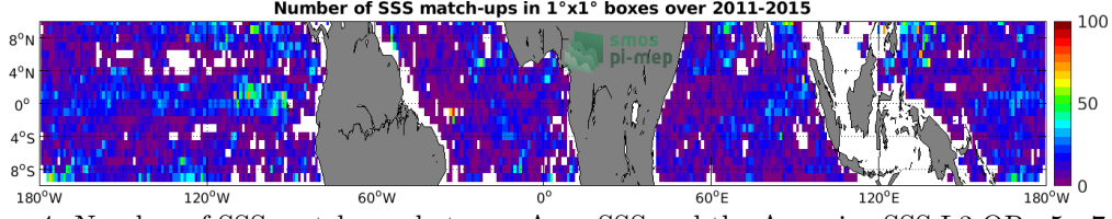
Figure 4: Number of SSS match-ups between Argo SSS and the Aquarius SSS L3 OR v5 - 7-Day running - Rain mask (NASA-GSFC) SSS product for the Equatorial Ocean 10N-10S Pi-MEP region over 1^\circ \times 1^\circ boxes and for the full satellite product period.
