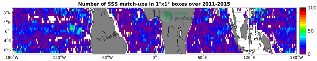
Figure 4: Number of SSS match-ups between Argo SSS and the Aquarius-L3-OR-V5-7DAY-RUNNING-RAIN-MASK-1DEG SSS product for the Equatorial Ocean 10N-10S Pi-MEP region over 1°x1° boxes and for the full satellite product period.
