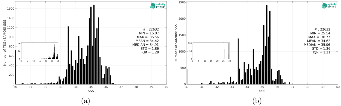
Figure 3: Histograms of SSS from TSG (SAMOS) (a) and Aquarius SSS L3 OR v5 - Monthly (NASA-GSFC) (b) considering all match-up pairs per bins of 0.1 over the Equatorial Ocean 10N-10S Pi-MEP region and for the full satellite product period.
