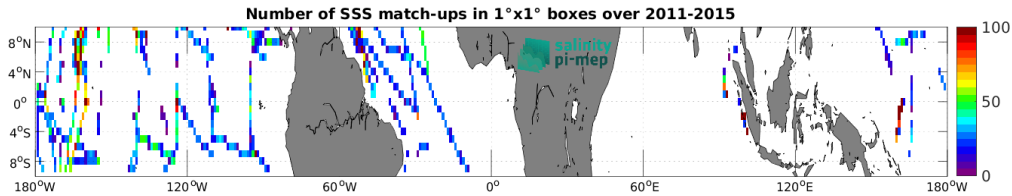
Figure 5: Number of SSS match-ups between TSG (SAMOS) SSS and the Aquarius SSS L3 OR v5 - Monthly (NASA-GSFC) SSS product for the Equatorial Ocean 10N-10S Pi-MEP region over 1^\circ \times 1^\circ boxes and for the full satellite product period.
