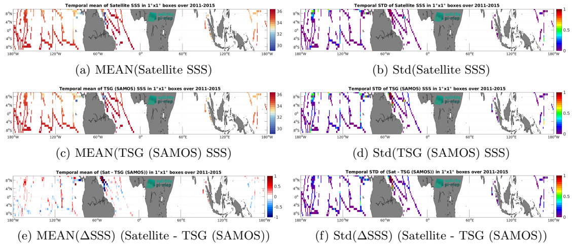
Figure 7: Temporal mean (left) and Std (right) of SSS from Aquarius SSS L3 OR v5 - Monthly (NASA-GSFC) (top), TSG (SAMOS) ( in situ ) dataset (middle), and of \Delta SSS (Satellite - TSG (SAMOS)). Only match-up pairs are used to generate these maps.
