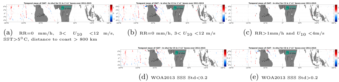
Figure 14: Temporal mean gridded over spatial boxes of size 1^\circ \times 1^\circ of \Delta SSS (Aquarius SSS L3 OR v5 - Monthly (NASA-GSFC) - TSG (SAMOS)) for 5 different subdatasets corresponding to: RR=0 mm/h, 3 < U_{10} < 12 m/s, SST>5°C, distance to coast > 800 km (a), RR=0 mm/h, 3 < U_{10} < 12 m/s (b), RR>1mm/h and U_{10} < 4 m/s (c), WOA2013 SSS Std<0.2 (d), WOA2013 SSS Std>0.2 (e).
