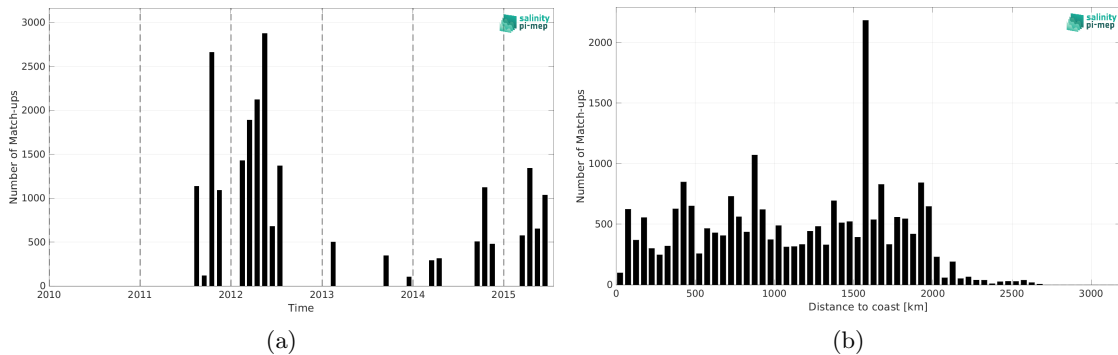
Figure 2: Number of match-ups between TSG (SAMOS) and Aquarius SSS L3 OR v5 - Monthly (NASA-GSFC) SSS as a function of time (a) and as function of the distance to coast (b) over the Equatorial Ocean 10N-10S Pi-MEP region and for the full satellite product period.
