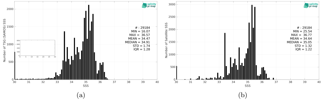
Figure 2: Histograms of SSS from TSG (SAMOS) (a) and Aquarius SSS L3 OR v5 - Monthly (NASA-GSFC) (b) considering all match-up pairs per bins of 0.1 over the Equatorial Ocean 10N-10S Pi-MEP region and for the full satellite product period.
