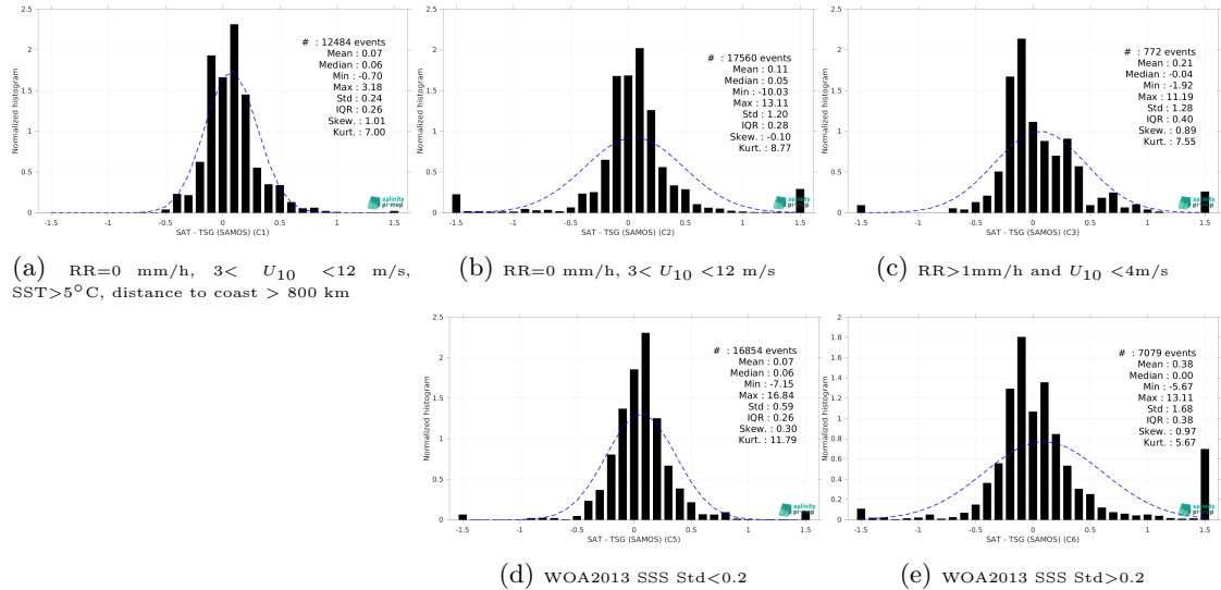
Figure 13: Normalized histogram of \Delta SSS (Aquarius SSS L3 OR v5 - Monthly (NASA-GSFC) - TSG (SAMOS)) for 5 different subdatasets corresponding to: RR=0 mm/h, 3 < U_{10} < 12 m/s, SST >5^\circ\text{C} , distance to coast > 800 km (a), RR=0 mm/h, 3 < U_{10} < 12 m/s (b), RR >1 mm/h and U_{10} < 4 m/s (c), WOA2013 SSS Std <0.2 (d), WOA2013 SSS Std >0.2 (e).
