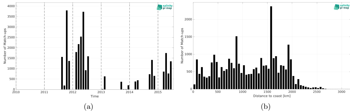
Figure 1: Number of match-ups between TSG (SAMOS) and Aquarius SSS L3 OR v5 - Monthly (NASA-GSFC) SSS as a function of time (a) and as function of the distance to coast (b) over the Equatorial Ocean 10N-10S Pi-MEP region and for the full satellite product period.
