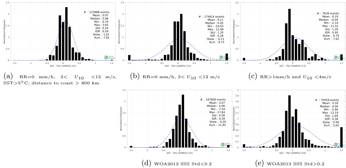
Figure 13: Normalized histogram of \Delta SSS (Aquarius SSS L3 OR v5 - Monthly (NASA-GSFC) - TSG (SAMOS)) for 5 different subdatasets corresponding to: RR=0 mm/h, 3 < U_{10} < 12 m/s, SST >5^\circ\text{C} , distance to coast > 800 km (a), RR=0 mm/h, 3 < U_{10} < 12 m/s (b), RR >1 mm/h and U_{10} < 4 m/s (c), WOA2013 SSS Std <0.2 (d), WOA2013 SSS Std >0.2 (e).
