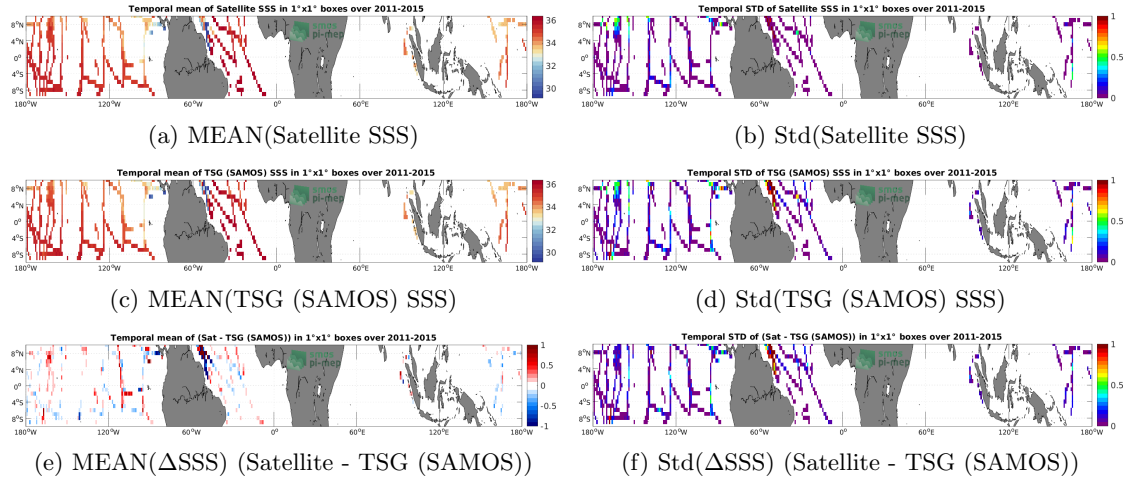
Figure 6: Temporal mean (left) and Std (right) of SSS from Aquarius SSS L3 OR v5 - Monthly (NASA-GSFC) (top), TSG (SAMOS) (middle), and of \Delta SSS (Satellite - TSG (SAMOS)). Only match-up pairs are used to generate these maps.
