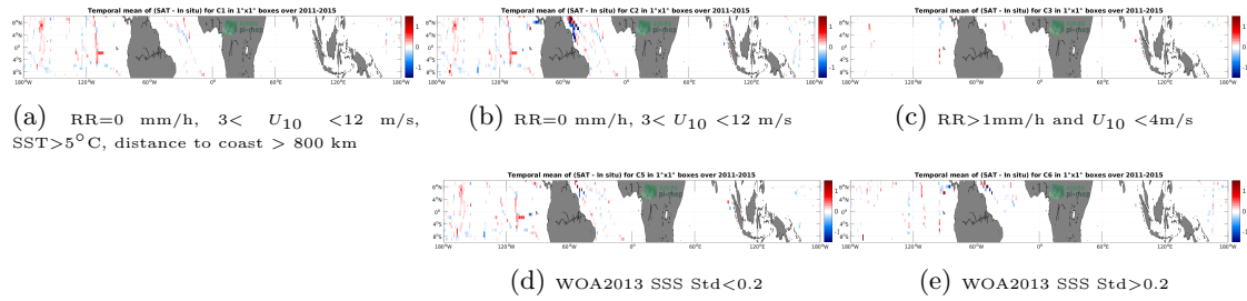
Figure 12: Temporal mean gridded over spatial boxes of size 1^\circ \times 1^\circ of \Delta SSS (Aquarius SSS L3 OR v5 - Monthly (NASA-GSFC) - TSG (SAMOS)) for 5 different subdatasets corresponding to: RR=0 mm/h, 3 < U_{10} < 12 m/s, SST >5^\circ\text{C} , distance to coast > 800 km (a), RR=0 mm/h, 3 < U_{10} < 12 m/s (b), RR >1 mm/h and U_{10} < 4 m/s (c), WOA2013 SSS Std <0.2 (d), WOA2013 SSS Std >0.2 (e).
