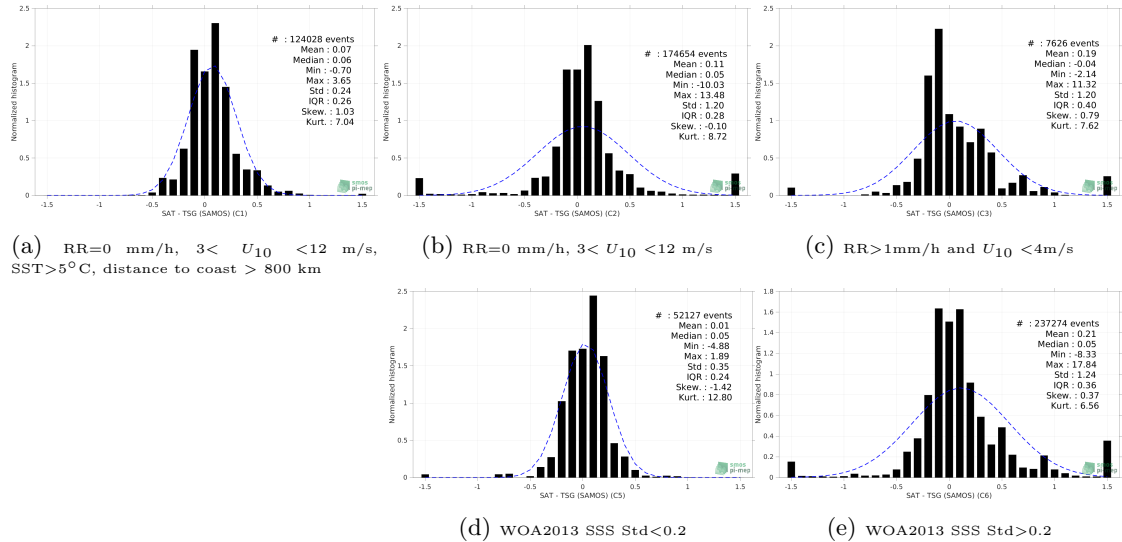
Figure 13: Normalized histogram of \Delta SSS (Aquarius SSS L3 OR v5 - Monthly (NASA-GSFC) - TSG (SAMOS)) for 5 different subdatasets corresponding to: RR=0 mm/h, 3 < U_{10} < 12 m/s, SST >5^\circ C, distance to coast > 800 km (a), RR=0 mm/h, 3 < U_{10} < 12 m/s (b), RR >1 mm/h and U_{10} < 4 m/s (c), WOA2013 SSS Std <0.2 (d), WOA2013 SSS Std >0.2 (e).
