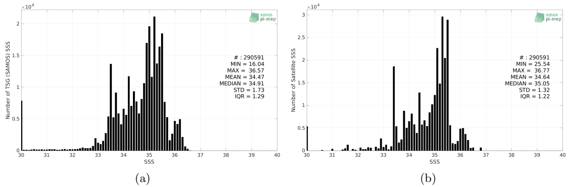
Figure 2: Histograms of SSS from TSG (SAMOS) (a) and Aquarius SSS L3 OR v5 - Monthly (NASA-GSFC) (b) considering all match-up pairs per bins of 0.1 over the Equatorial Ocean 10N-10S Pi-MEP region and for the full satellite product period.
