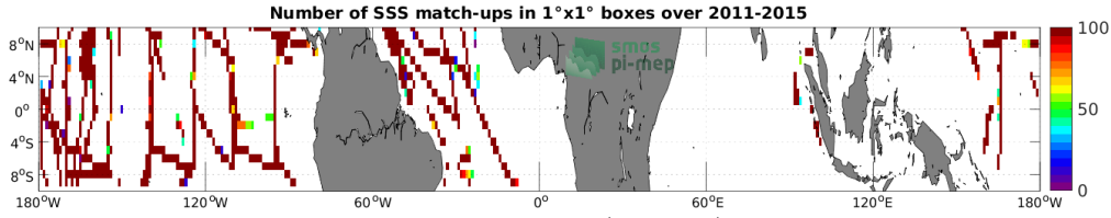
Figure 4: Number of SSS match-ups between TSG (SAMOS) SSS and the Aquarius SSS L3 OR v5 - Monthly (NASA-GSFC) SSS product for the Equatorial Ocean 10N-10S Pi-MEP region over 1^\circ \times 1^\circ boxes and for the full satellite product period.
