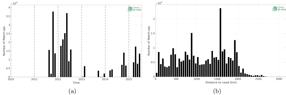
Figure 1: Number of match-ups between TSG (SAMOS) and Aquarius SSS L3 OR v5 - Monthly (NASA-GSFC) SSS as a function of time (a) and as function of the distance to coast (b) over the Equatorial Ocean 10N-10S Pi-MEP region and for the full satellite product period.
