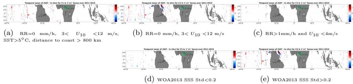
Figure 12: Temporal mean gridded over spatial boxes of size 1^\circ \times 1^\circ of \Delta SSS (Aquarius SSS L3 OR v5 - Monthly (NASA-GSFC) - TSG (SAMOS)) for 5 different subdatasets corresponding to:RR=0 mm/h, 3 < U_{10} < 12 m/s, SST >5^\circ C, distance to coast > 800 km (a), RR=0 mm/h, 3 < U_{10} < 12 m/s (b), RR >1 mm/h and U_{10} < 4 m/s (c), WOA2013 SSS Std <0.2 (d), WOA2013 SSS Std >0.2 (e).
