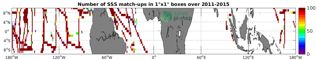
Figure 4: Number of SSS match-ups between TSG-SAMOS SSS and the Aquarius-L3-OR-V5-MONTHLY-1DEG SSS product for the Equatorial Ocean 10N-10S Pi-MEP region over 1^\circ \times 1^\circ boxes and for the full satellite product period.
