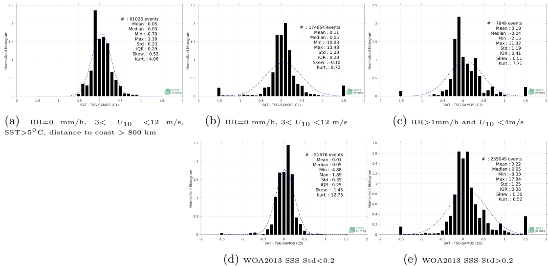
Figure 13: Normalized histogram of \Delta SSS (Aquarius-L3-OR-V5-MONTHLY-1DEG - TSG-SAMOS) for 5 different subdatasets corresponding to: RR=0 mm/h, 3 < U_{10} < 12 m/s, SST >5^\circ C, distance to coast > 800 km (a), RR=0 mm/h, 3 < U_{10} < 12 m/s (b), RR >1 mm/h and U_{10} < 4 m/s (c), WOA2013 SSS Std <0.2 (d), WOA2013 SSS Std >0.2 (e).
