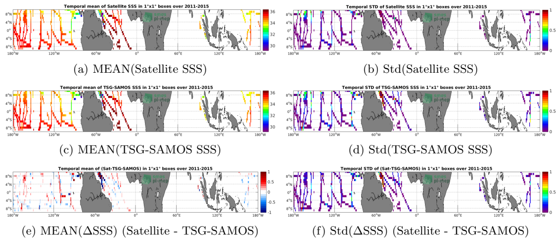
Figure 6: Temporal mean (left) and Std (right) of SSS from Aquarius-L3-OR-V5-MONTHLY-1DEG (top), TSG-SAMOS (middle), and of \Delta SSS (Satellite - TSG-SAMOS). Only match-up pairs are used to generate these maps.
