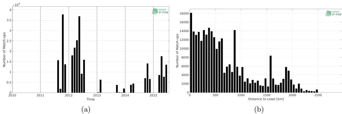
Figure 1: Number of match-ups between TSG-SAMOS and Aquarius-L3-OR-V5-MONTHLY-1DEG SSS as a function of time (a) and as function of the distance to coast (b) over the Equatorial Ocean 10N-10S Pi-MEP region and for the full satellite product period.
