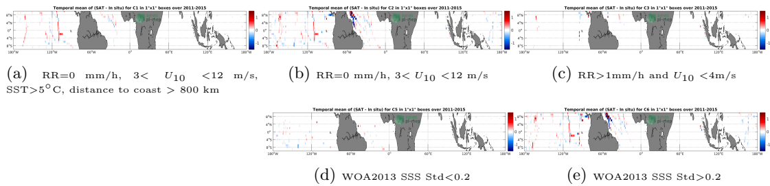
Figure 12: Temporal mean gridded over spatial boxes of size 1^\circ \times 1^\circ of \Delta SSS (Aquarius-L3-OR-V5-MONTHLY-1DEG - TSG-SAMOS) for 5 different subdatasets corresponding to: RR=0 mm/h, 3 < U_{10} < 12 m/s, SST >5^\circ C, distance to coast > 800 km (a), RR=0 mm/h, 3 < U_{10} < 12 m/s (b), RR >1 mm/h and U_{10} < 4 m/s (c), WOA2013 SSS Std <0.2 (d), WOA2013 SSS Std >0.2 (e).
