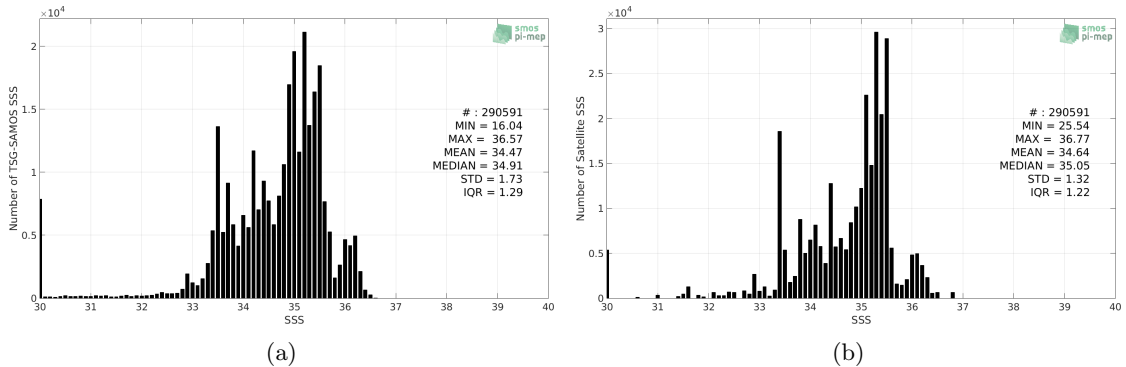
Figure 2: Histograms of SSS from TSG-SAMOS (a) and Aquarius-L3-OR-V5-MONTHLY-1DEG (b) considering all match-up pairs per bins of 0.1 over the Equatorial Ocean 10N-10S Pi-MEP region and for the full satellite product period.
