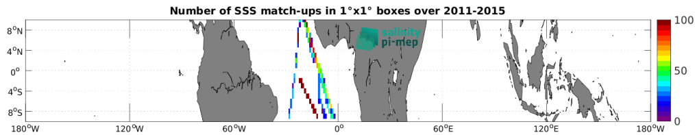
Figure 5: Number of SSS match-ups between TSG (Polarstern) SSS and the Aquarius SSS L3 OR v5 - Monthly (NASA-GSFC) SSS product for the Equatorial Ocean 10N-10S Pi-MEP region over 1^\circ \times 1^\circ boxes and for the full satellite product period.
