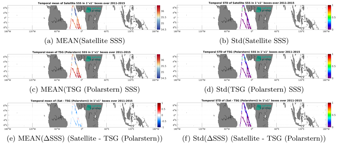
Figure 7: Temporal mean (left) and Std (right) of SSS from Aquarius SSS L3 OR v5 - Monthly (NASA-GSFC) (top), TSG (Polarstern) (middle), and of \Delta SSS (Satellite - TSG (Polarstern)). Only match-up pairs are used to generate these maps.
