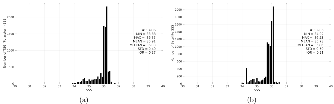
Figure 3: Histograms of SSS from TSG (Polarstern) (a) and Aquarius SSS L3 OR v5 - Monthly (NASA-GSFC) (b) considering all match-up pairs per bins of 0.1 over the Equatorial Ocean 10N-10S Pi-MEP region and for the full satellite product period.
