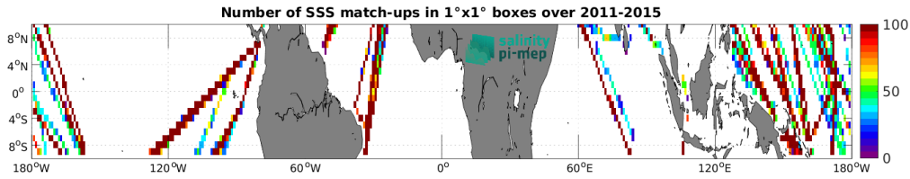
Figure 5: Number of SSS match-ups between TSG (LEGOS-DM) SSS and the Aquarius SSS L3 OR v5 - Monthly (NASA-GSFC) SSS product for the Equatorial Ocean 10N-10S Pi-MEP region over 1^\circ \times 1^\circ boxes and for the full satellite product period.
