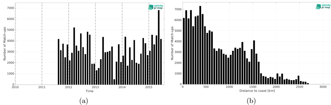
Figure 2: Number of match-ups between TSG (LEGOS-DM) and Aquarius SSS L3 OR v5 - Monthly (NASA-GSFC) SSS as a function of time (a) and as function of the distance to coast (b) over the Equatorial Ocean 10N-10S Pi-MEP region and for the full satellite product period.
