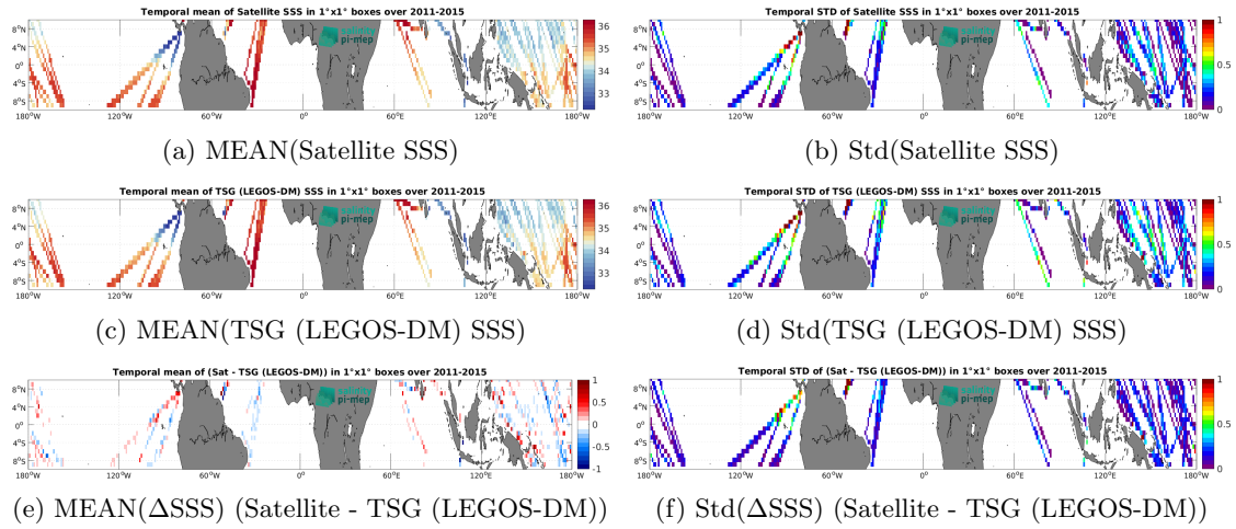
Figure 7: Temporal mean (left) and Std (right) of SSS from Aquarius SSS L3 OR v5 - Monthly (NASA-GSFC) (top), TSG (LEGOS-DM) (middle), and of \Delta SSS (Satellite - TSG (LEGOS-DM)). Only match-up pairs are used to generate these maps.
