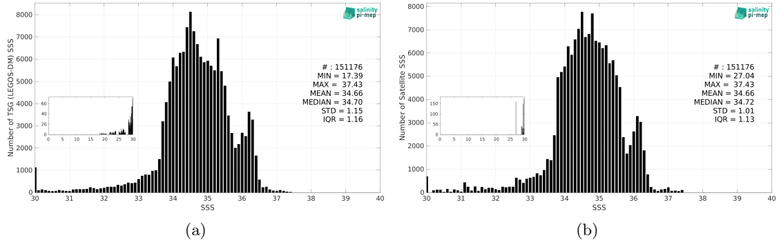
Figure 3: Histograms of SSS from TSG (LEGOS-DM) (a) and Aquarius SSS L3 OR v5 - Monthly (NASA-GSFC) (b) considering all match-up pairs per bins of 0.1 over the Equatorial Ocean 10N-10S Pi-MEP region and for the full satellite product period.
