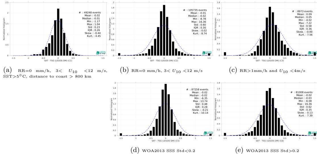
Figure 13: Normalized histogram of \Delta SSS (Aquarius SSS L3 OR v5 - Monthly (NASA-GSFC) - TSG (LEGOS-DM)) for 5 different subdatasets corresponding to: RR=0 mm/h, 3 < U_{10} < 12 m/s, SST >5^\circ C, distance to coast > 800 km (a), RR=0 mm/h, 3 < U_{10} < 12 m/s (b), RR >1 mm/h and U_{10} < 4 m/s (c), WOA2013 SSS Std <0.2 (d), WOA2013 SSS Std >0.2 (e).
