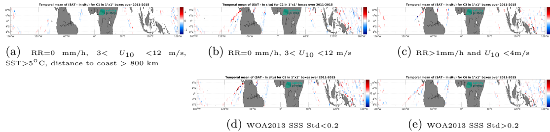
Figure 12: Temporal mean gridded over spatial boxes of size 1^\circ \times 1^\circ of \Delta SSS (Aquarius SSS L3 OR v5 - Monthly (NASA-GSFC) - TSG (LEGOS-DM)) for 5 different subdatasets corresponding to: RR=0 mm/h, 3 < U_{10} < 12 m/s, SST >5^\circ C, distance to coast > 800 km (a), RR=0 mm/h, 3 < U_{10} < 12 m/s (b), RR >1 mm/h and U_{10} < 4 m/s (c), WOA2013 SSS Std <0.2 (d), WOA2013 SSS Std >0.2 (e).
