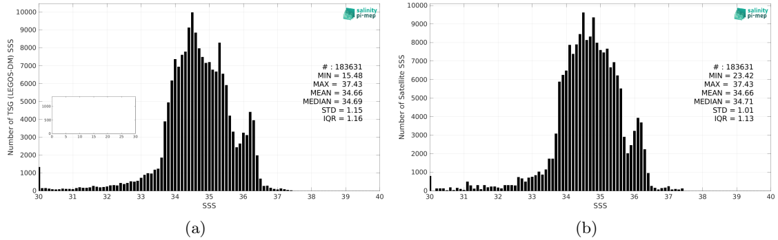
Figure 2: Histograms of SSS from TSG (LEGOS-DM) (a) and Aquarius SSS L3 OR v5 - Monthly (NASA-GSFC) (b) considering all match-up pairs per bins of 0.1 over the Equatorial Ocean 10N-10S Pi-MEP region and for the full satellite product period.
