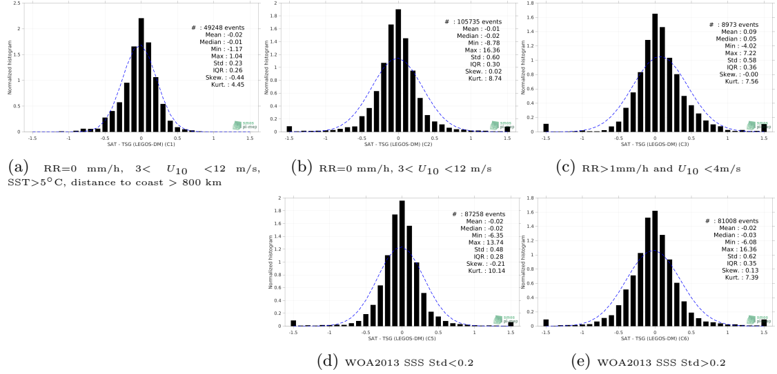
Figure 13: Normalized histogram of \Delta\text{SSS} (Aquarius SSS L3 OR v5 - Monthly (NASA-GSFC) - TSG (LEGOS-DM)) for 5 different subdatasets corresponding to: RR=0 mm/h, 3 < U_{10} < 12 m/s, SST>5°C, distance to coast > 800 km (a), RR=0 mm/h, 3 < U_{10} < 12 m/s (b), RR>1mm/h and U_{10} < 4 m/s (c), WOA2013 SSS Std<0.2 (d), WOA2013 SSS Std>0.2 (e).
