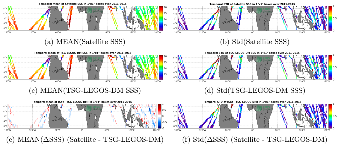
Figure 6: Temporal mean (left) and Std (right) of SSS from Aquarius-L3-OR-V5-MONTHLY-1DEG (top), TSG-LEGOS-DM (middle), and of \Delta SSS (Satellite - TSG-LEGOS-DM). Only match-up pairs are used to generate these maps.
