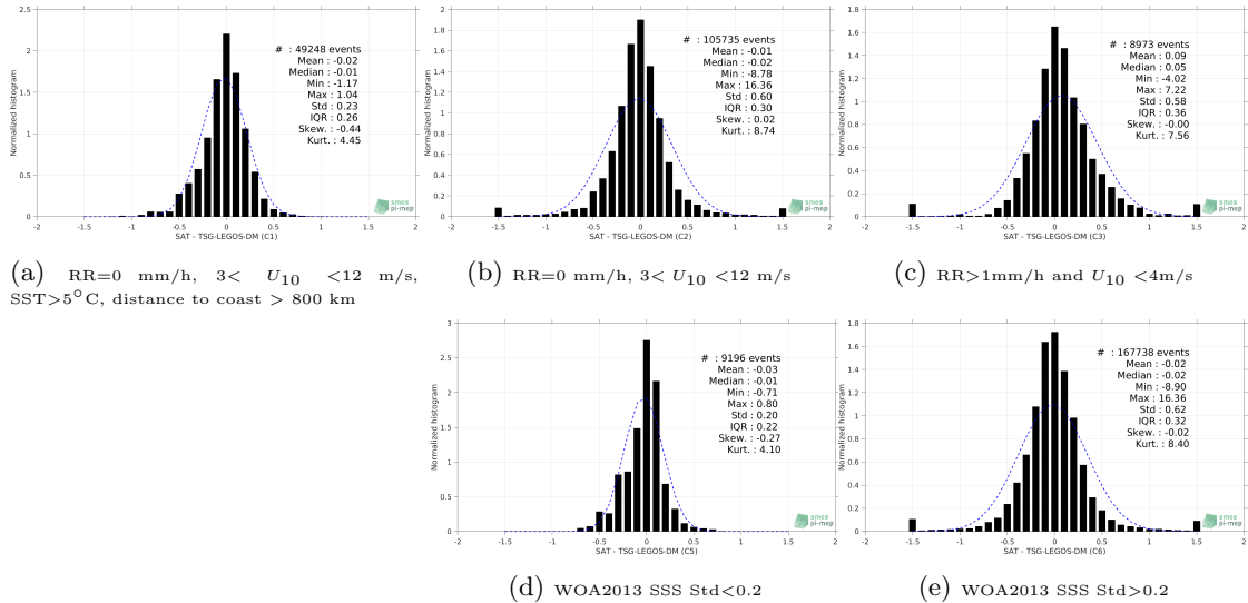
Figure 13: Normalized histogram of ΔSSS (Aquarius-L3-OR-V5-MONTHLY-1DEG - TSG-LEGOS-DM) for 5 different subdatasets corresponding to: RR=0 mm/h, 3 < U_{10} < 12 m/s, SST>5°C, distance to coast > 800 km (a), RR=0 mm/h, 3 < U_{10} < 12 m/s (b), RR>1mm/h and U_{10} < 4 m/s (c), WOA2013 SSS Std<0.2 (d), WOA2013 SSS Std>0.2 (e).
