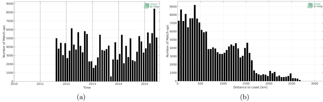
Figure 1: Number of match-ups between TSG-LEGOS-DM and Aquarius-L3-OR-V5-MONTHLY-1DEG SSS as a function of time (a) and as function of the distance to coast (b) over the Equatorial Ocean 10N-10S Pi-MEP region and for the full satellite product period.
