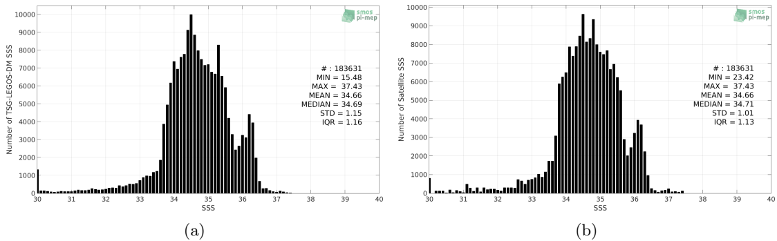
Figure 2: Histograms of SSS from TSG-LEGOS-DM (a) and Aquarius-L3-OR-V5-MONTHLY-1DEG (b) considering all match-up pairs per bins of 0.1 over the Equatorial Ocean 10N-10S Pi-MEP region and for the full satellite product period.
