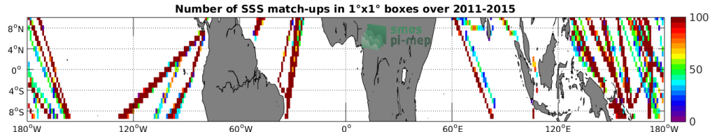
Figure 4: Number of SSS match-ups between TSG-LEGOS-DM SSS and the Aquarius-L3-OR-V5-MONTHLY-1DEG SSS product for the Equatorial Ocean 10N-10S Pi-MEP region over 1°x1° boxes and for the full satellite product period.
