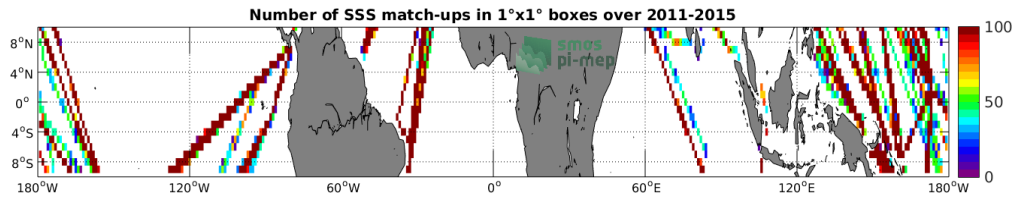
Figure 4: Number of SSS match-ups between TSG-LEGOS-DM SSS and the Aquarius-L3-OR-V5-MONTHLY-1DEG SSS product for the Equatorial Ocean 10N-10S Pi-MEP region over 1^\circ \times 1^\circ boxes and for the full satellite product period.
