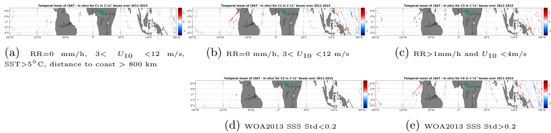
Figure 12: Temporal mean gridded over spatial boxes of size 1^\circ \times 1^\circ of \Delta SSS (Aquarius-L3-OR-V5-MONTHLY-1DEG - TSG-LEGOS-DM) for 5 different subdatasets corresponding to:RR=0 mm/h, 3 < U_{10} < 12 m/s, SST >5^\circ C, distance to coast > 800 km (a), RR=0 mm/h, 3 < U_{10} < 12 m/s (b), RR >1 mm/h and U_{10} < 4 m/s (c), WOA2013 SSS Std <0.2 (d), WOA2013 SSS Std >0.2 (e).
