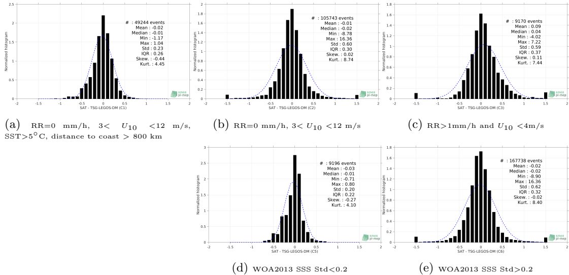
Figure 13: Normalized histogram of \Delta SSS (Aquarius-L3-OR-V5-MONTHLY-1DEG - TSG-LEGOS-DM) for 5 different subdatasets corresponding to: RR=0 mm/h, 3 < U_{10} < 12 m/s, SST >5^\circ C, distance to coast > 800 km (a), RR=0 mm/h, 3 < U_{10} < 12 m/s (b), RR >1 mm/h and U_{10} < 4 m/s (c), WOA2013 SSS Std <0.2 (d), WOA2013 SSS Std >0.2 (e).
