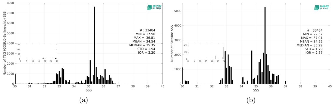
Figure 3: Histograms of SSS from TSG (GOSUD-Sailing-ship) (a) and Aquarius SSS L3 OR v5 - Monthly (NASA-GSFC) (b) considering all match-up pairs per bins of 0.1 over the Equatorial Ocean 10N-10S Pi-MEP region and for the full satellite product period.
