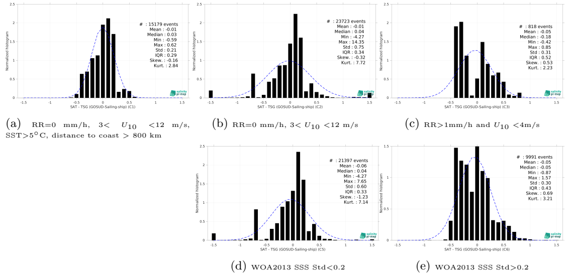
Figure 15: Normalized histogram of \Delta SSS (Aquarius SSS L3 OR v5 - Monthly (NASA-GSFC) - TSG (GOSUD-Sailing-ship)) for 5 different subdatasets corresponding to: RR=0 mm/h, 3 < U_{10} < 12 m/s, SST>5°C, distance to coast > 800 km (a), RR=0 mm/h, 3 < U_{10} < 12 m/s (b), RR>1mm/h and U_{10} < 4 m/s (c), WOA2013 SSS Std<0.2 (d), WOA2013 SSS Std>0.2 (e).
