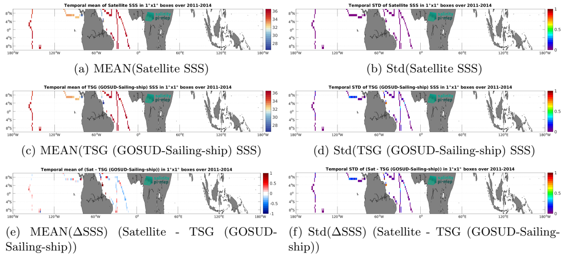
Figure 7: Temporal mean (left) and Std (right) of SSS from Aquarius SSS L3 OR v5 - Monthly (NASA-GSFC) (top), TSG (GOSUD-Sailing-ship) (middle), and of \Delta SSS (Satellite - TSG (GOSUD-Sailing-ship)). Only match-up pairs are used to generate these maps.
