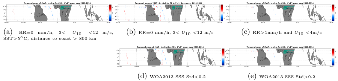
Figure 14: Temporal mean gridded over spatial boxes of size 1^\circ \times 1^\circ of \Delta SSS (Aquarius SSS L3 OR v5 - Monthly (NASA-GSFC) - TSG (GOSUD-Sailing-ship)) for 5 different subdatasets corresponding to: RR=0 mm/h, 3 < U_{10} < 12 m/s, SST>5°C, distance to coast > 800 km (a), RR=0 mm/h, 3 < U_{10} < 12 m/s (b), RR>1mm/h and U_{10} < 4 m/s (c), WOA2013 SSS Std<0.2 (d), WOA2013 SSS Std>0.2 (e).
