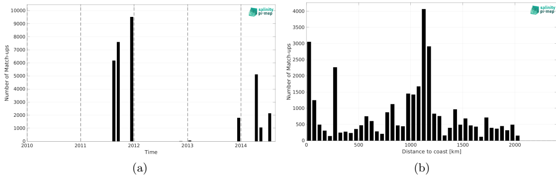
Figure 2: Number of match-ups between TSG (GOSUD-Sailing-ship) and Aquarius SSS L3 OR v5 - Monthly (NASA-GSFC) SSS as a function of time (a) and as function of the distance to coast (b) over the Equatorial Ocean 10N-10S Pi-MEP region and for the full satellite product period.
