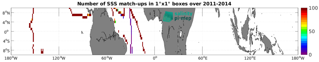
Figure 4: Number of SSS match-ups between TSG (GOSUD-Sailing-ship) SSS and the Aquarius SSS L3 OR v5 - Monthly (NASA-GSFC) SSS product for the Equatorial Ocean 10N-10S Pi-MEP region over 1^\circ \times 1^\circ boxes and for the full satellite product period.
