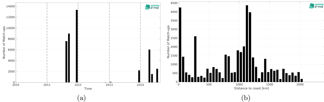
Figure 1: Number of match-ups between TSG (GOSUD-Sailing-ship) and Aquarius SSS L3 OR v5 - Monthly (NASA-GSFC) SSS as a function of time (a) and as function of the distance to coast (b) over the Equatorial Ocean 10N-10S Pi-MEP region and for the full satellite product period.
