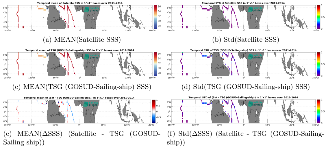
Figure 6: Temporal mean (left) and Std (right) of SSS from Aquarius SSS L3 OR v5 - Monthly (NASA-GSFC) (top), TSG (GOSUD-Sailing-ship) (middle), and of \Delta SSS (Satellite - TSG (GOSUD-Sailing-ship)). Only match-up pairs are used to generate these maps.
